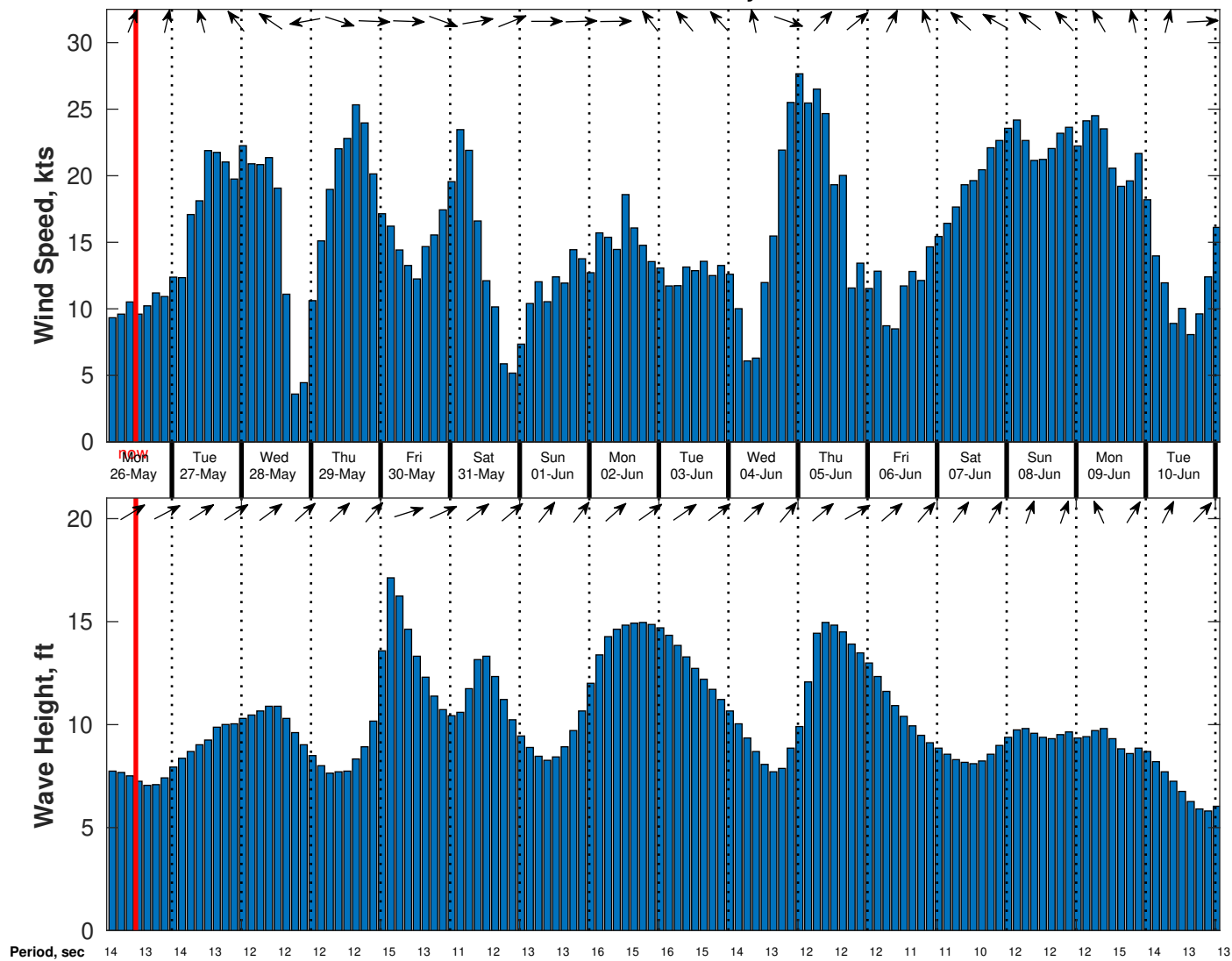
Wind & Wave Forecast for Benthic Solutions South Africa HF Site2 from 25-May-2025 02:00:00 to 10-Jun-2025 02:00:00
