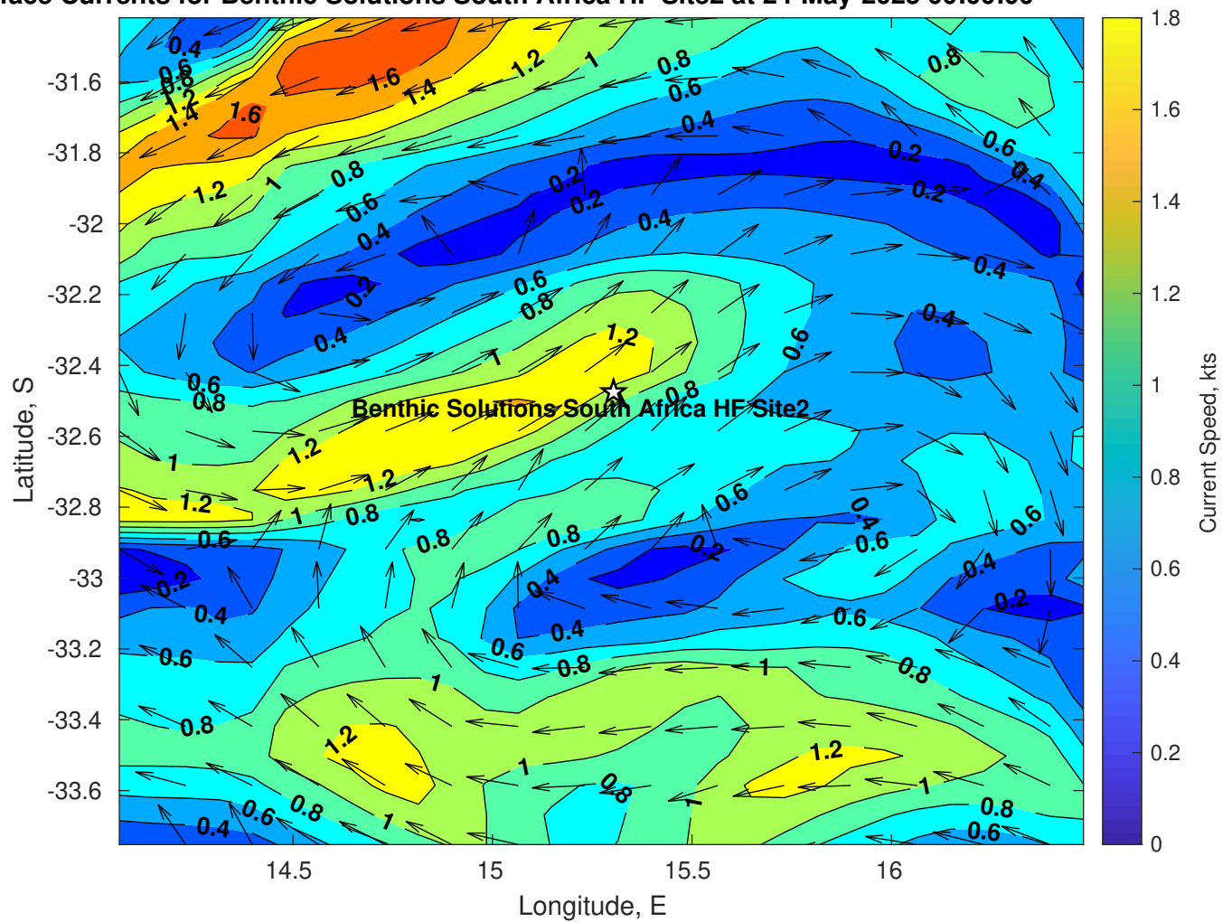
Surface Currents for Benthic Solutions South Africa HF Site2 at 24-May-2025 00:00:00
