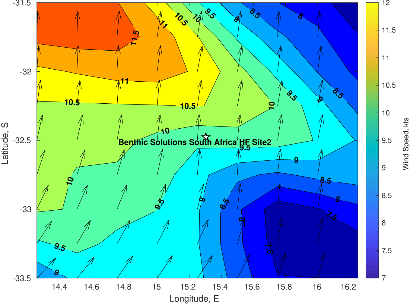
Winds (kts) for Benthic Solutions South Africa HF Site2 at 25-May-2025 09:00:00
