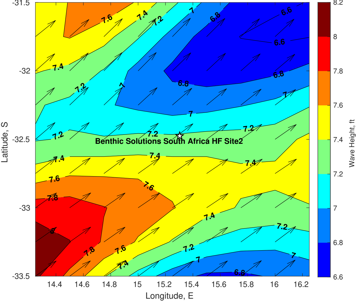
Wave Height (ft) for Benthic Solutions South Africa HF Site2 at 25-May-2025 09:00:00
