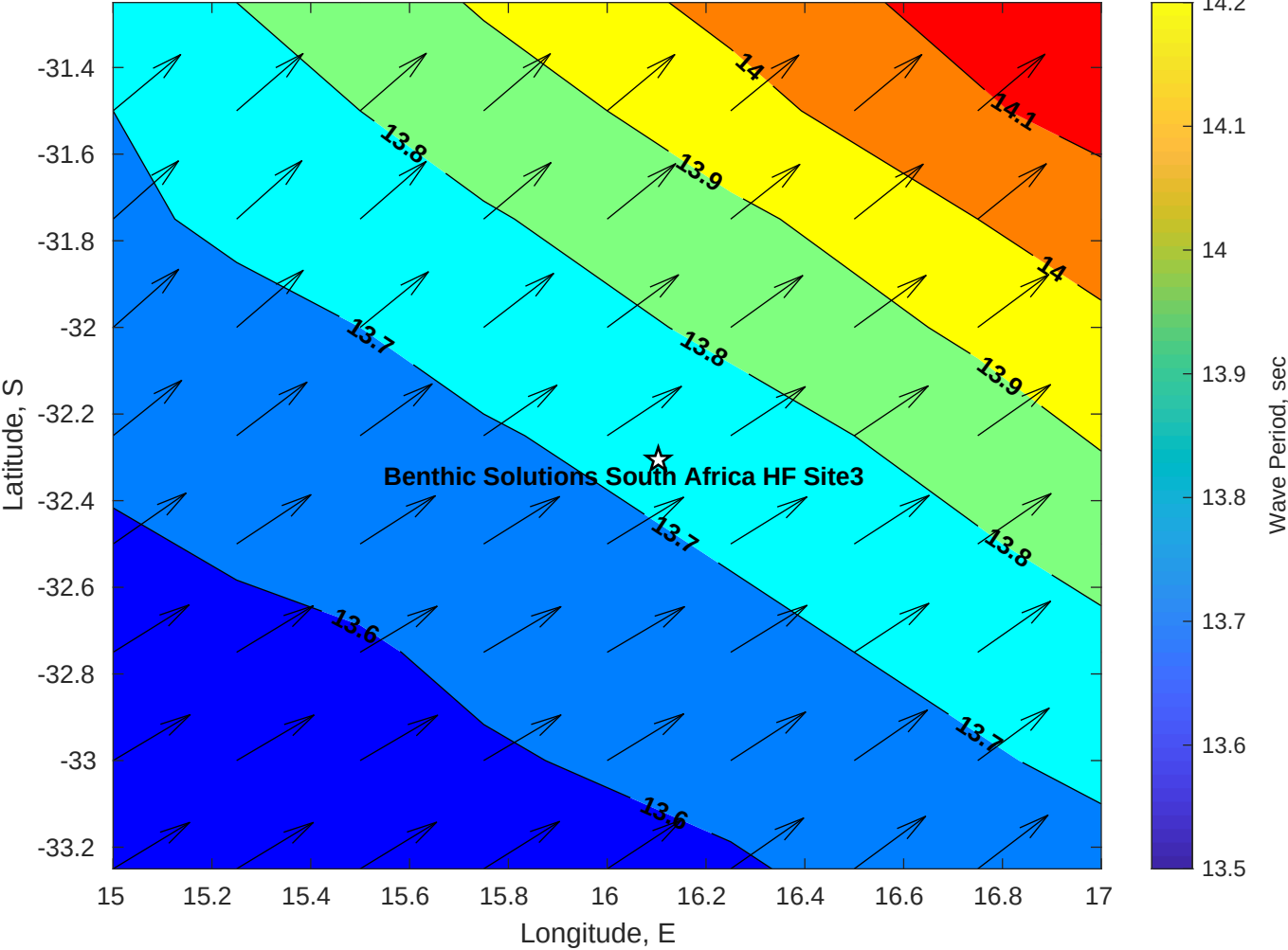
Wave Period (sec) for Benthic Solutions South Africa HF Site3 at 25-May-2025 09:00:00
