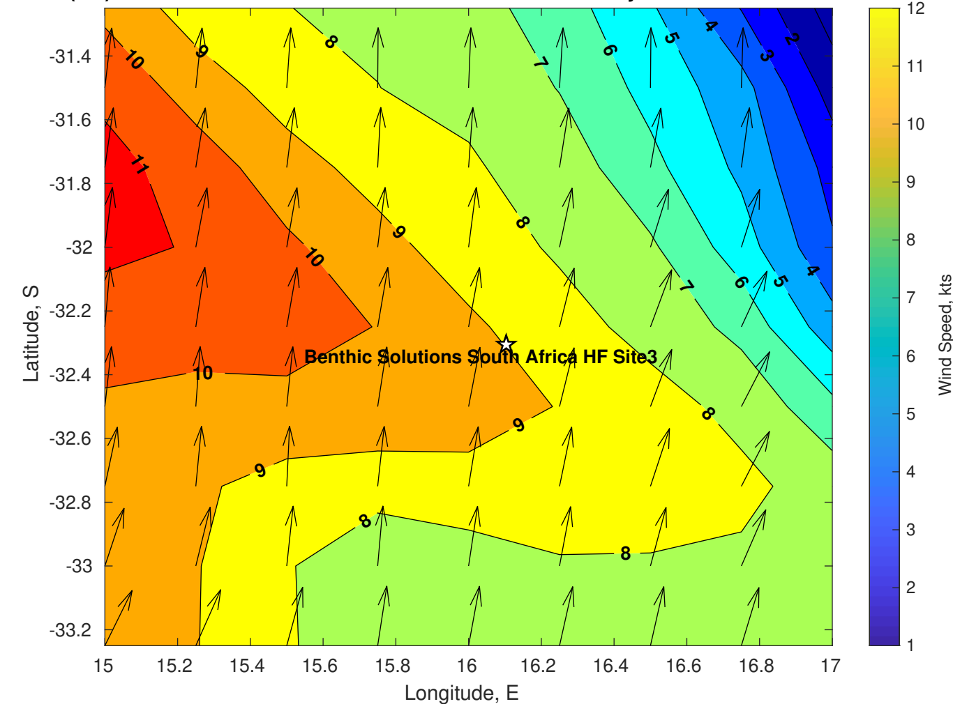
Winds (kts) for Benthic Solutions South Africa HF Site3 at 25-May-2025 09:00:00
