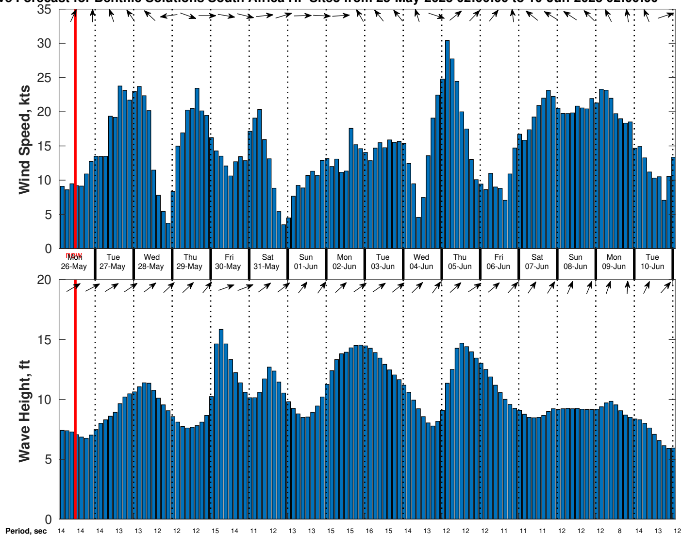
Wind & Wave Forecast for Benthic Solutions South Africa HF Site3 from 25-May-2025 02:00:00 to 10-Jun-2025 02:00:00
