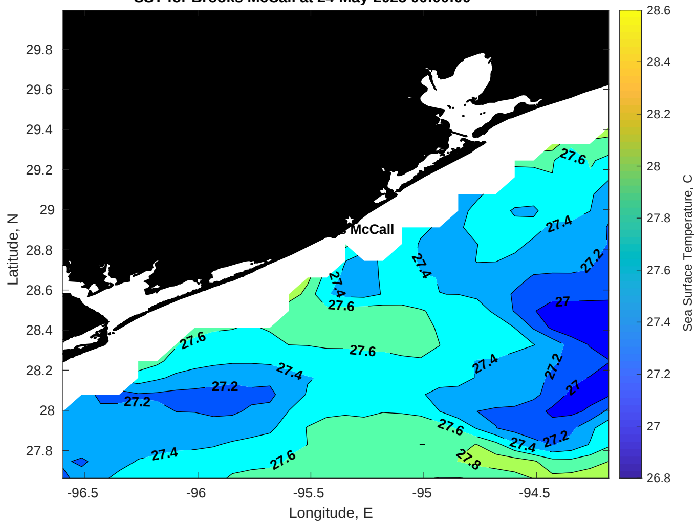
SST for Brooks McCall at 24-May-2025 00:00:00
