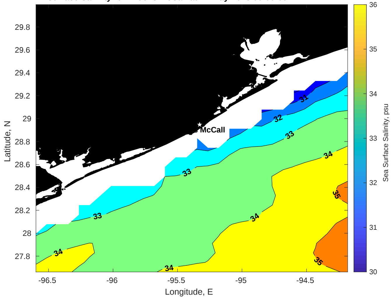
Surface Salinity for Brooks McCall at 24-May-2025 00:00:00
