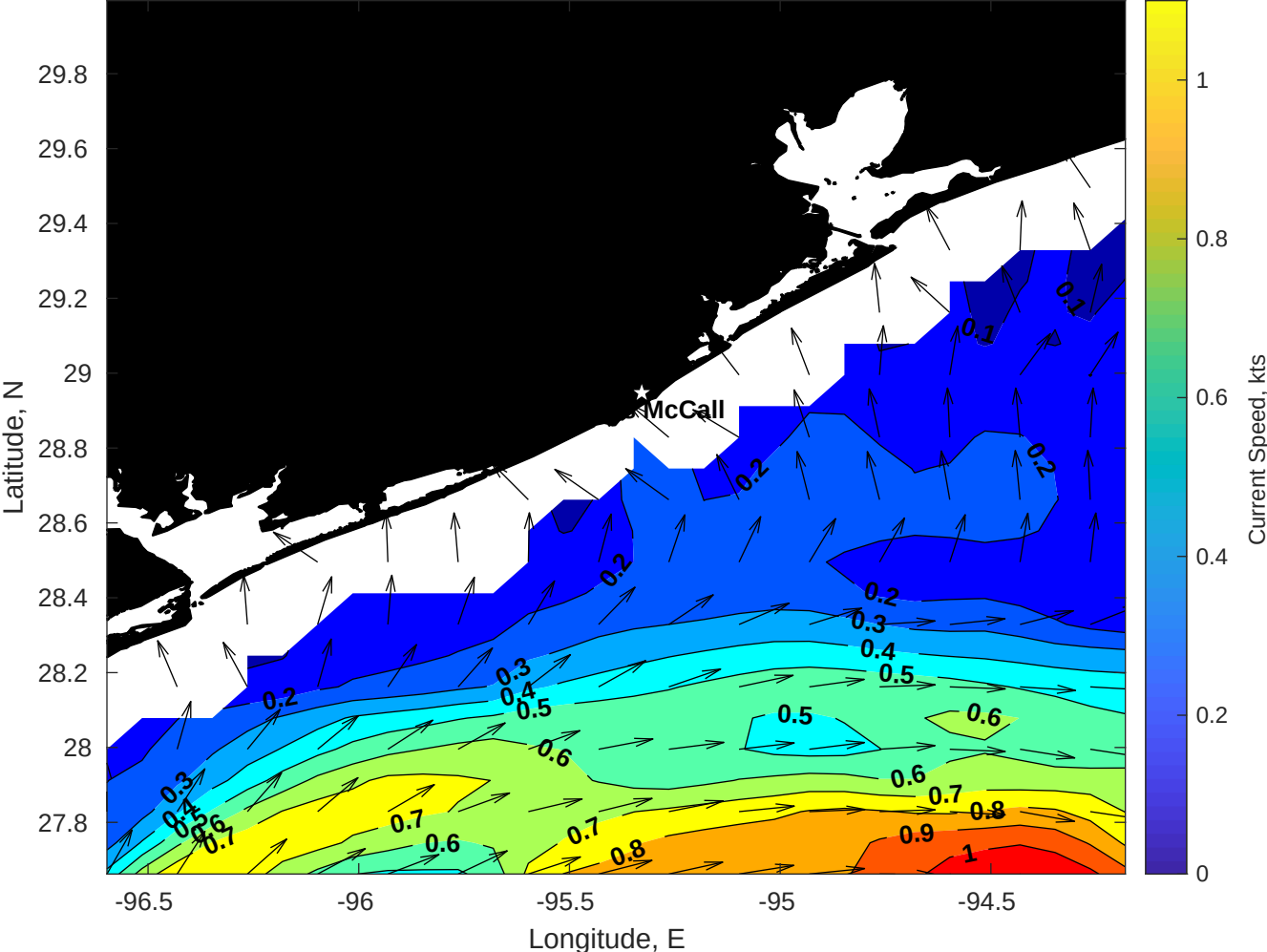
Surface Currents for Brooks McCall at 24-May-2025 00:00:00
