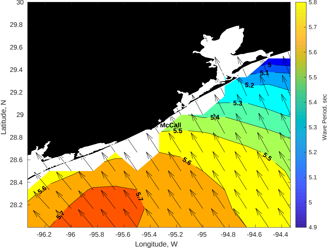
Wave Period (sec) for Brooks McCall at 25-May-2025 09:00:00
