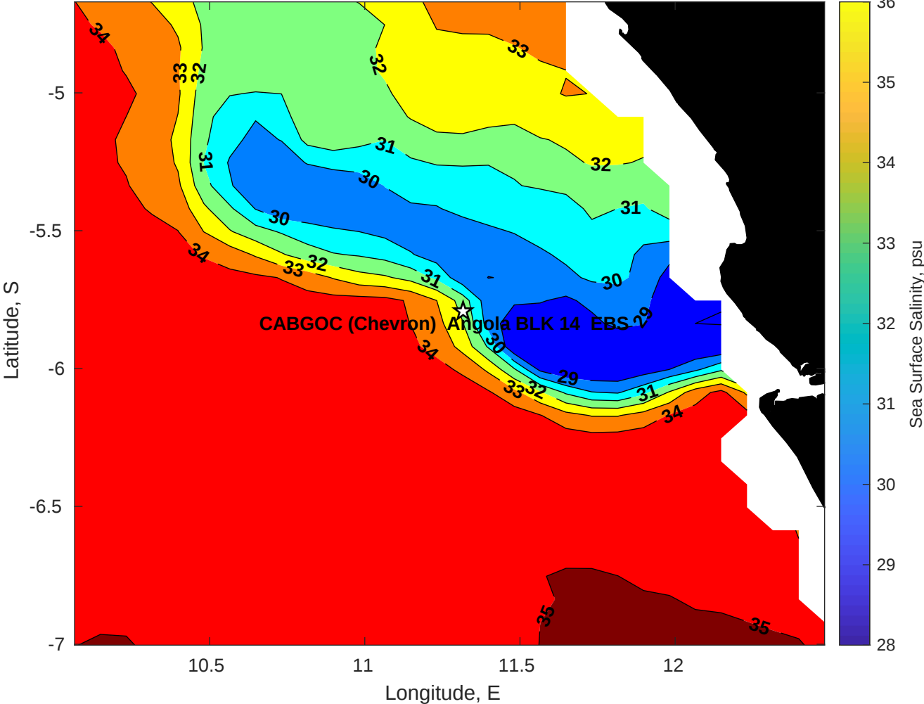
Surface Salinity for CABGOC (Chevron) Angola BLK 14 EBS at 24-May-2025 00:00:00
