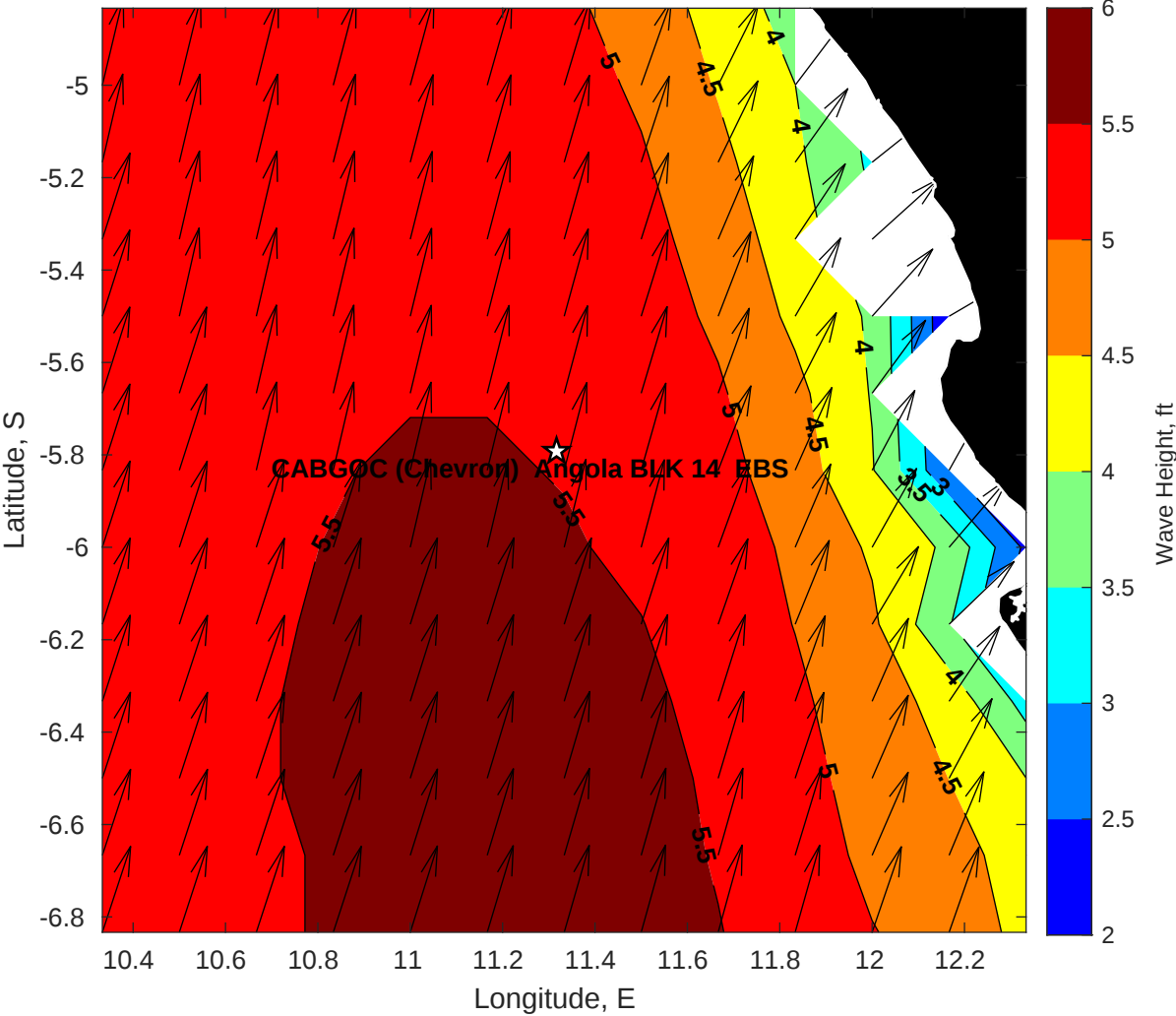
Wave Height (ft) for CABGOC (Chevron) Angola BLK 14 EBS at 25-May-2025 09:00:00
