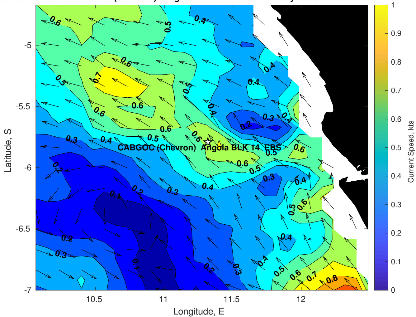
Surface Currents for CABGOC (Chevron) Angola BLK 14 EBS at 24-May-2025 00:00:00
