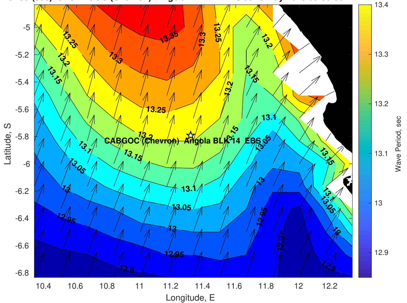
Wave Period (sec) for CABGOC (Chevron) Angola BLK 14 EBS at 25-May-2025 09:00:00
