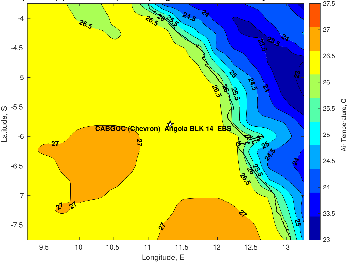
Air Temperature (C) for CABGOC (Chevron) Angola BLK 14 EBS at 25-May-2025
