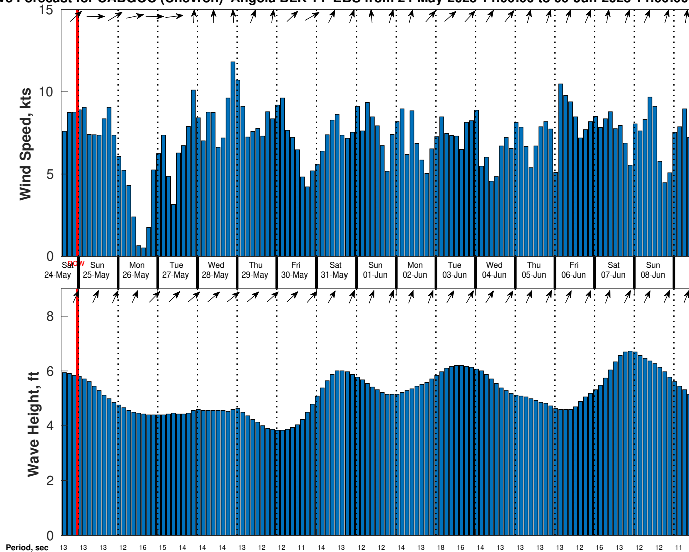
Wind & Wave Forecast for CABGOC (Chevron) Angola BLK 14 EBS from 24-May-2025 14:00:00 to 09-Jun-2025 14:00:00
