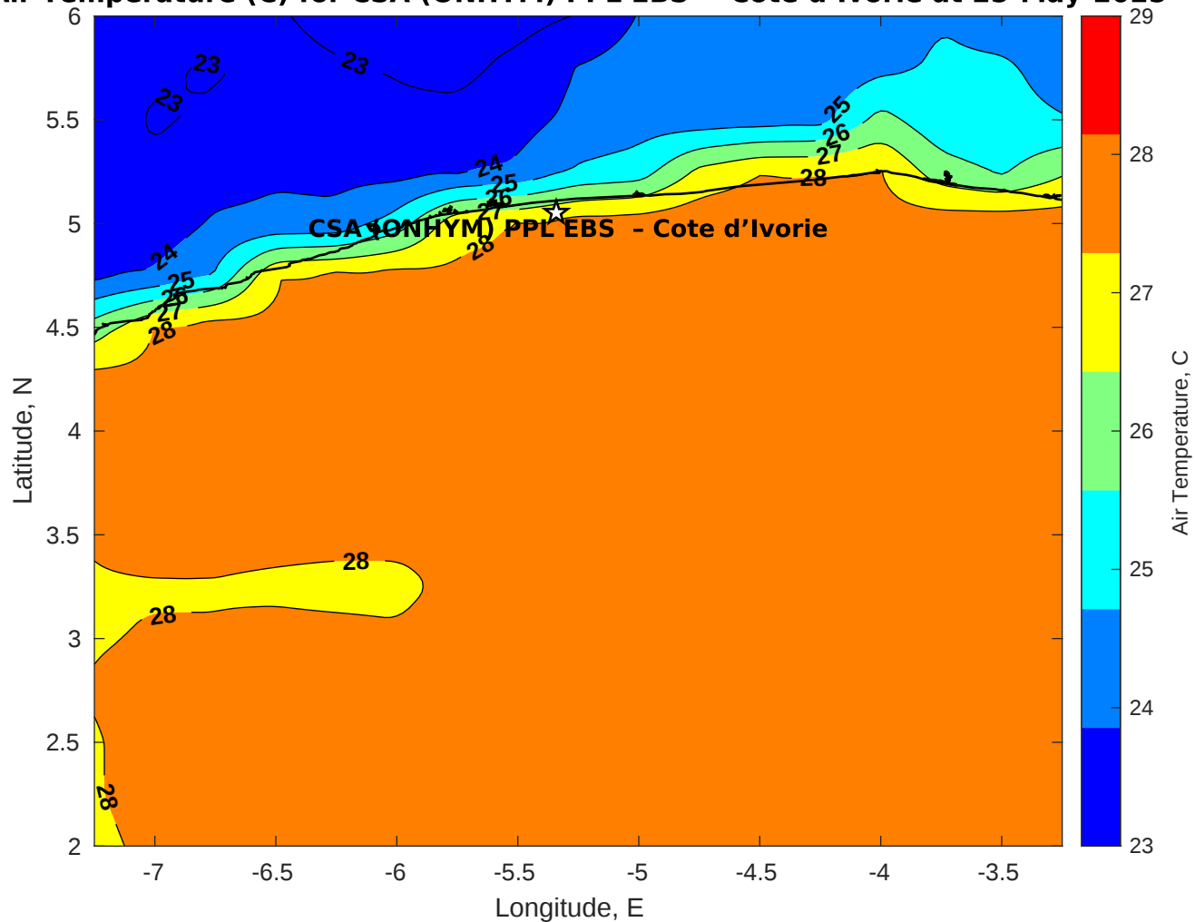
Air Temperature (C) for CSA (ONHYM) PPL EBS - Cote d'Ivoire at 25-May-2025
