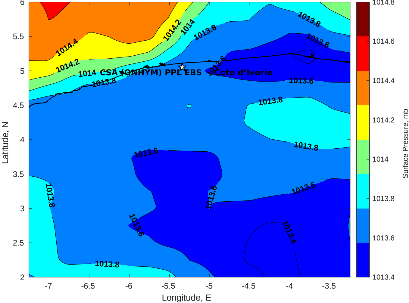
Surface Pressure (mb) for CSA (ONHYM) PPL EBS - Cote d'Ivoire at 27-May-2025 00:00:00
