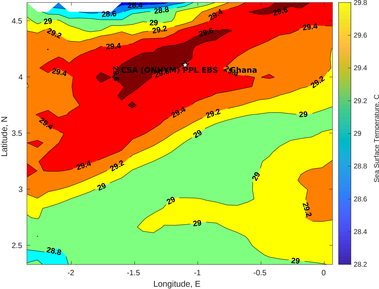
SST for CSA (ONHYM) PPL EBS - Ghana at 24-May-2025 00:00:00
