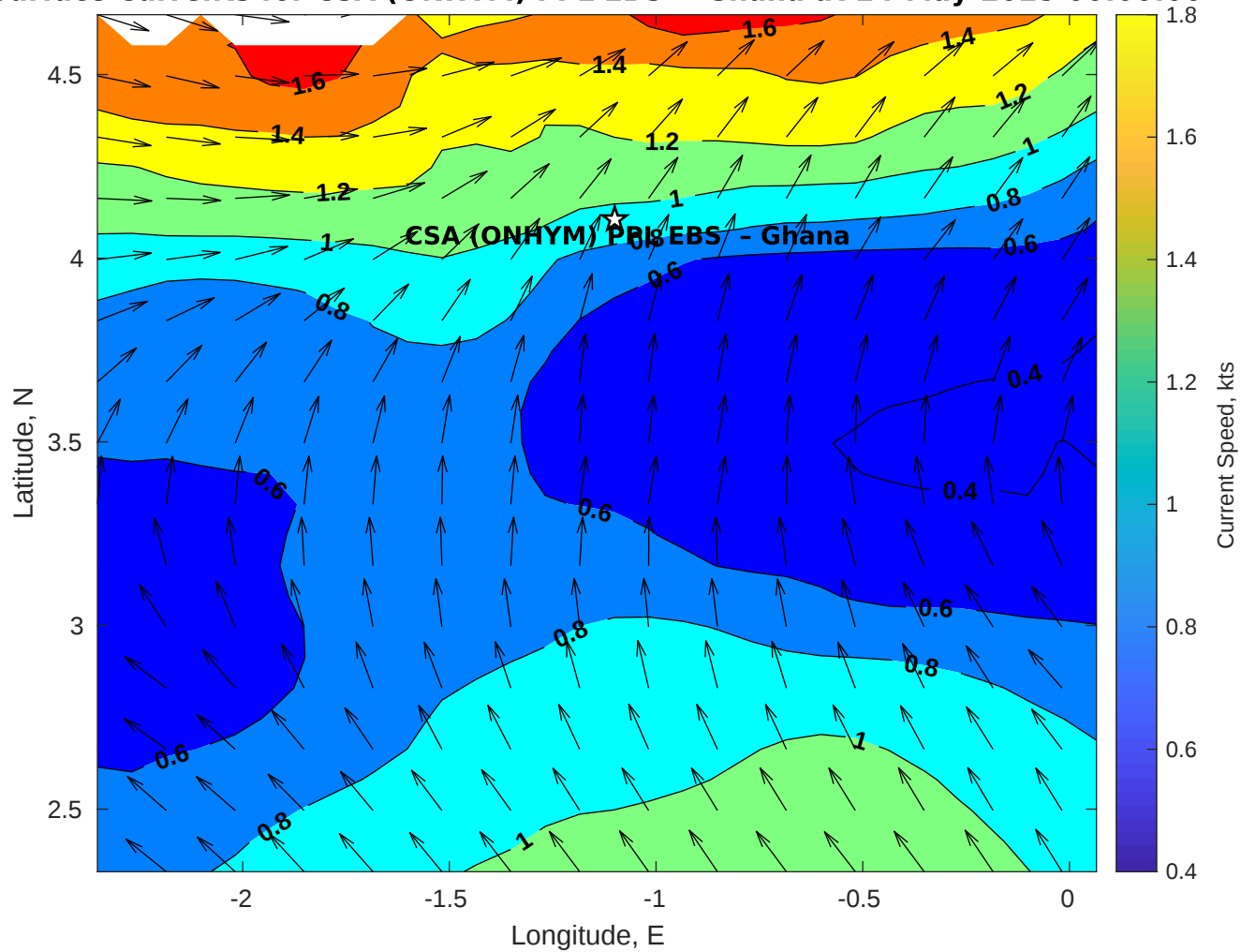
Surface Currents for CSA (ONHYM) PPL EBS - Ghana at 24-May-2025 00:00:00
