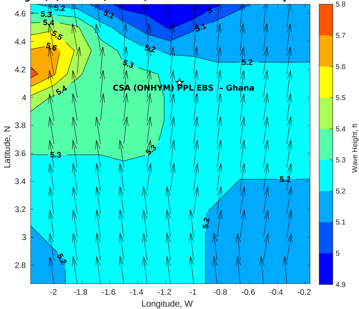
Wave Height (ft) for CSA (ONHYM) PPL EBS - Ghana at 25-May-2025 09:00:00
