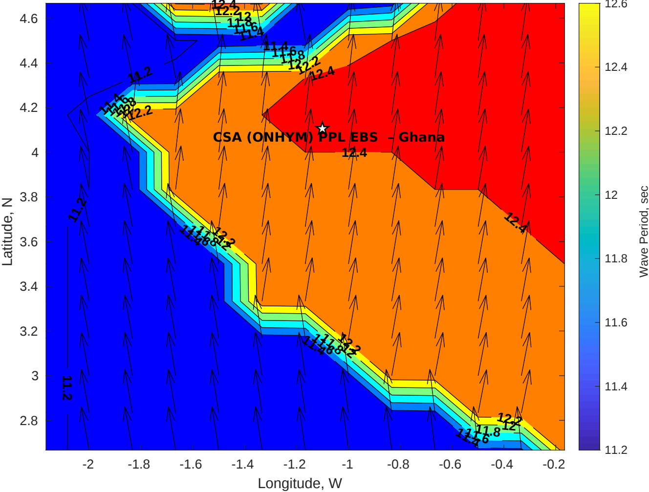
Wave Period (sec) for CSA (ONHYM) PPL EBS - Ghana at 25-May-2025 09:00:00
