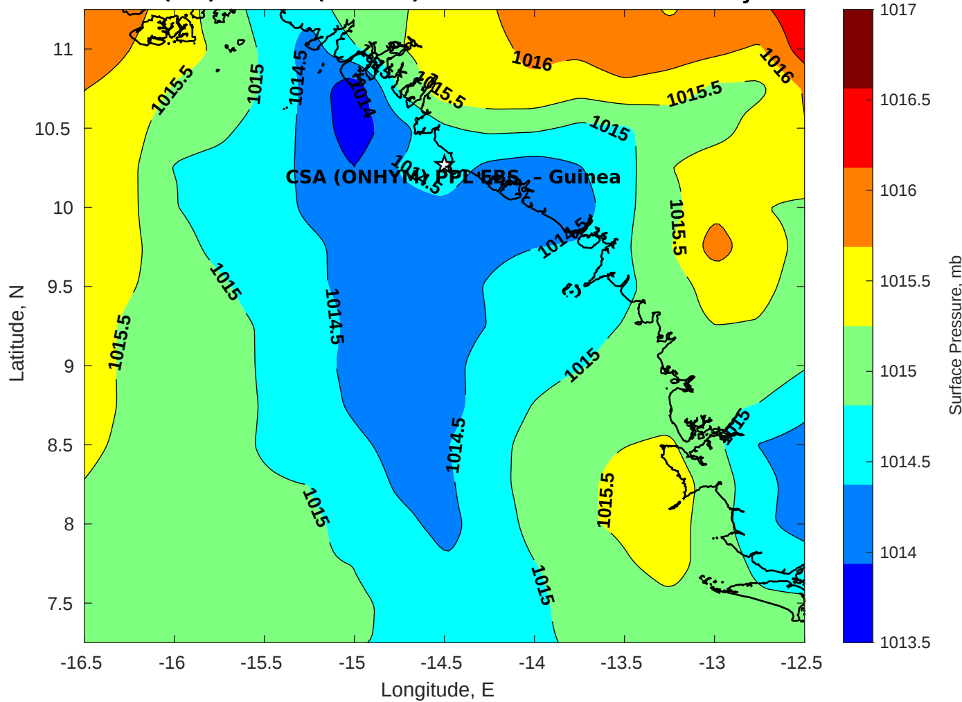
Surface Pressure (mb) for CSA (ONHYM) PPL EBS - Guinea at 25-May-2025 00:00:00
