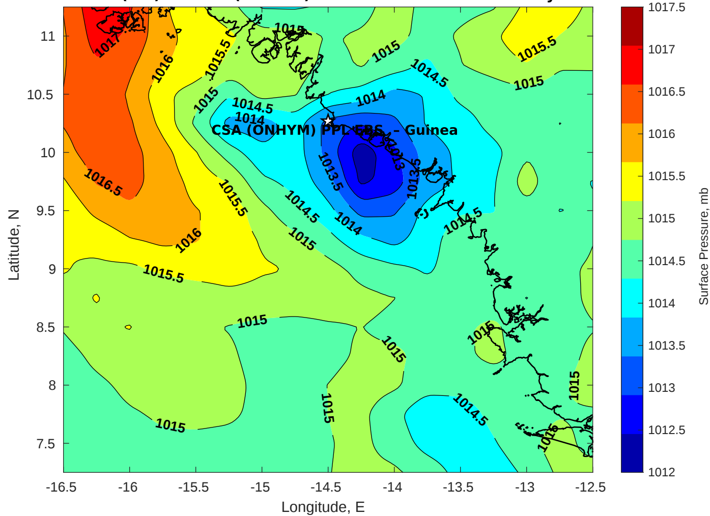
Surface Pressure (mb) for CSA (ONHYM) PPL EBS - Guinea at 26-May-2025 00:00:00
