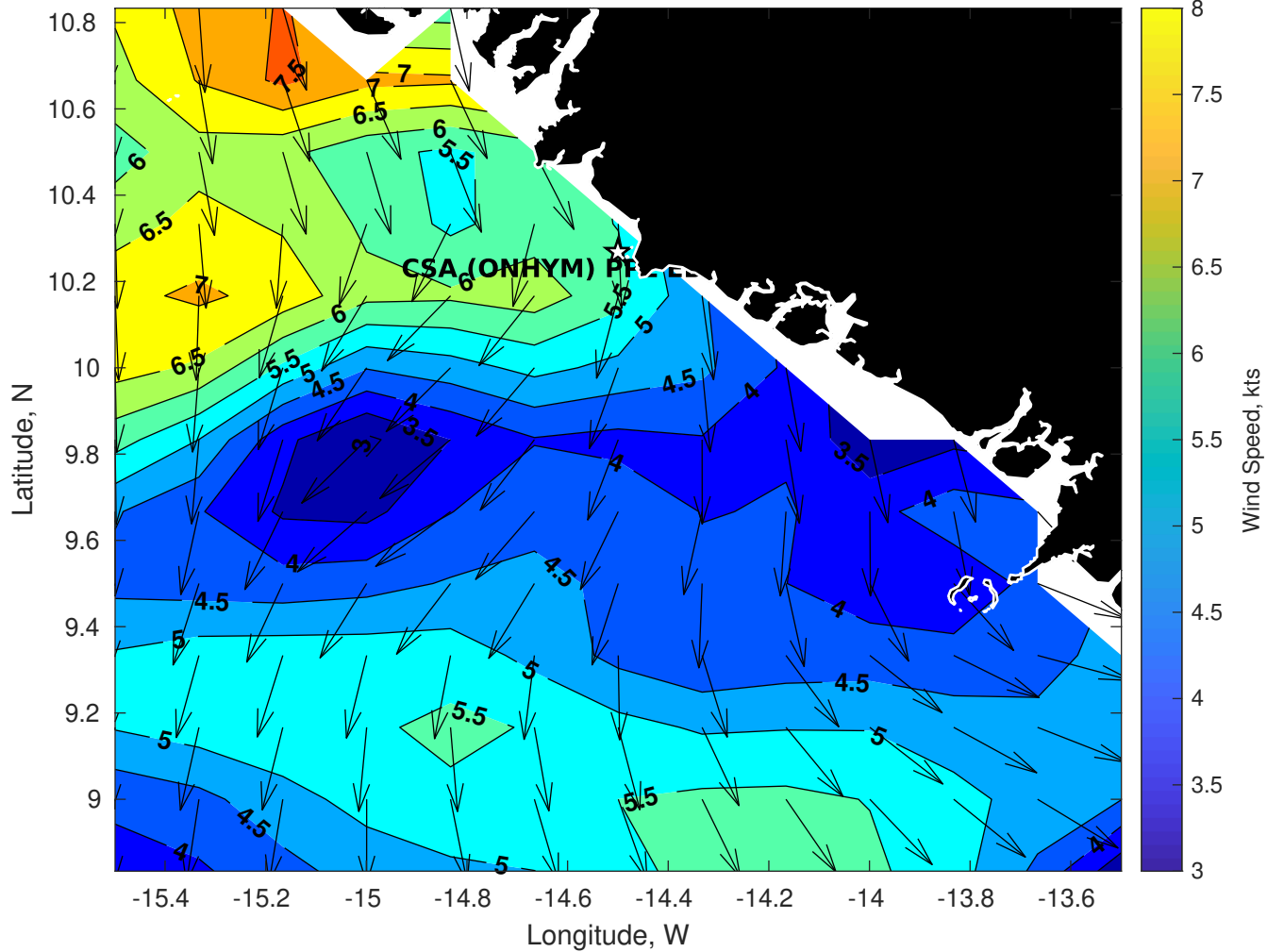
Winds (kts) for CSA (ONHYM) PPL EBS - Guinea at 25-May-2025 09:00:00
