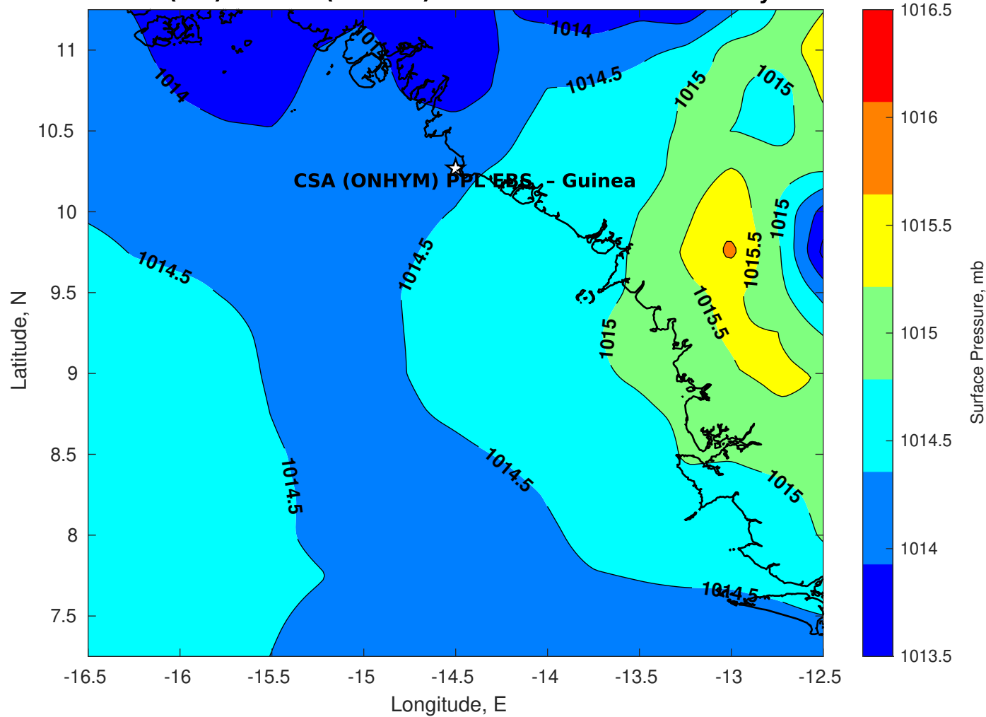
Surface Pressure (mb) for CSA (ONHYM) PPL EBS - Guinea at 27-May-2025 00:00:00
