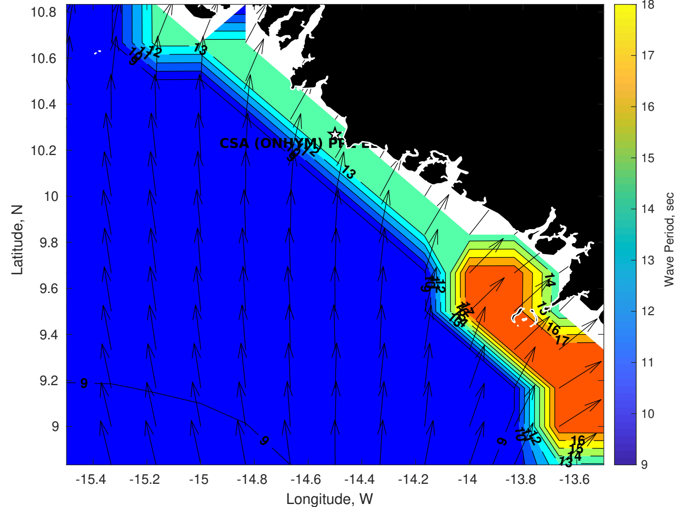
Wave Period (sec) for CSA (ONHYM) PPL EBS - Guinea at 25-May-2025 09:00:00
