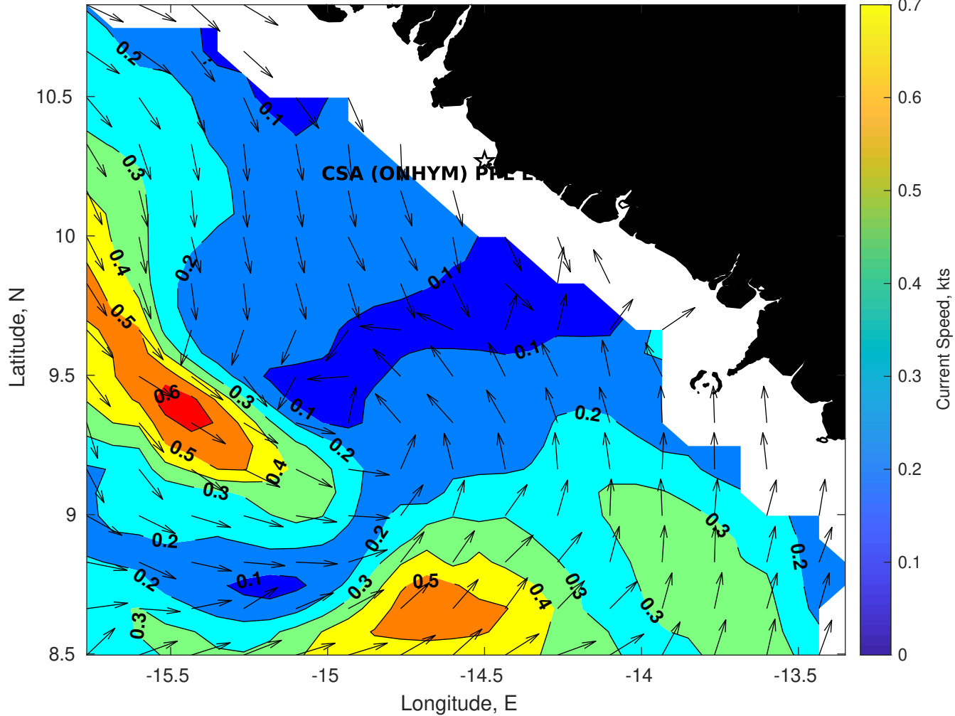
Surface Currents for CSA (ONHYM) PPL EBS - Guinea at 24-May-2025 00:00:00
