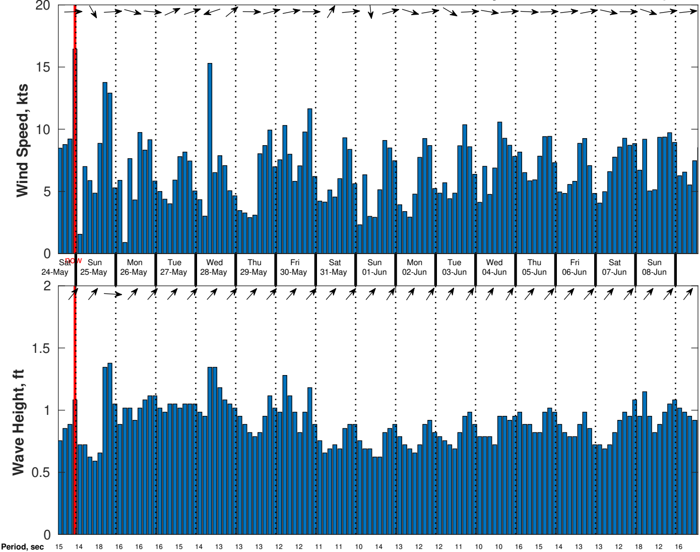
Wind & Wave Forecast for CSA (ONHYM) PPL EBS - Guinea from 24-May-2025 13:00:00 to 09-Jun-2025 13:00:00
