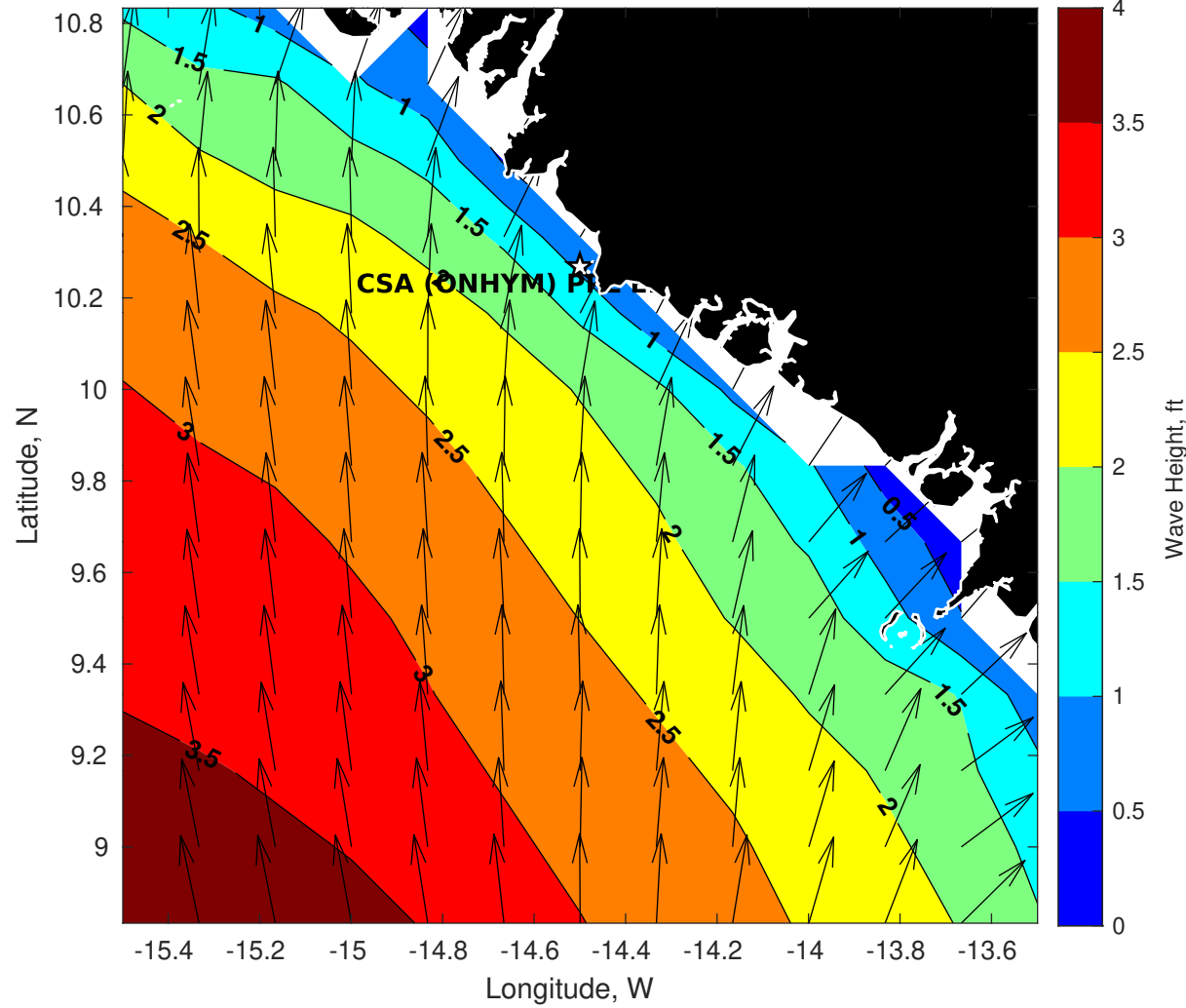
Wave Height (ft) for CSA (ONHYM) PPL EBS - Guinea at 25-May-2025 09:00:00
