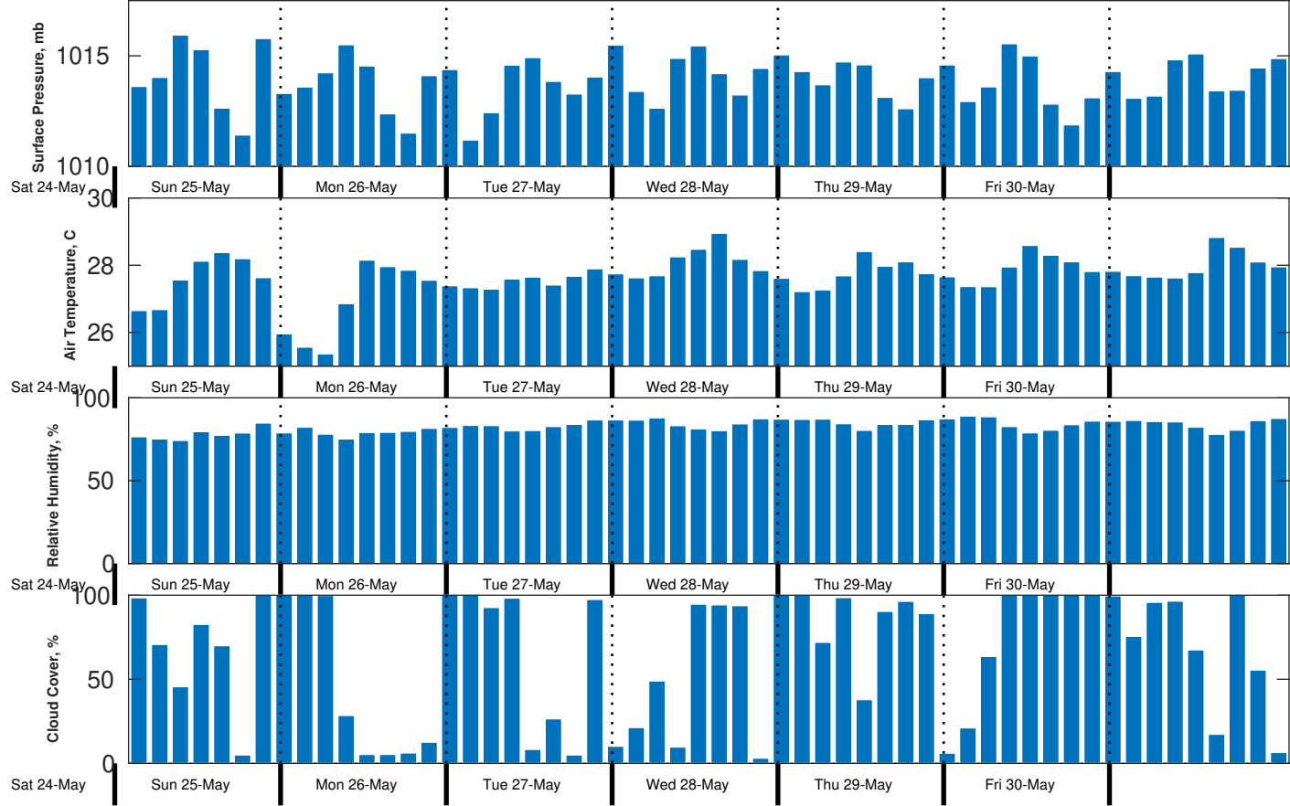
Met Forecast for CSA (ONHYM) PPL EBS - Guinea from 25-May-2025 00:00:00 to 01-Jun-2025 00:00:00
