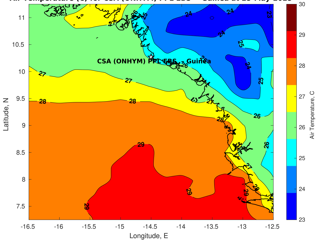
Air Temperature (C) for CSA (ONHYM) PPL EBS - Guinea at 25-May-2025
