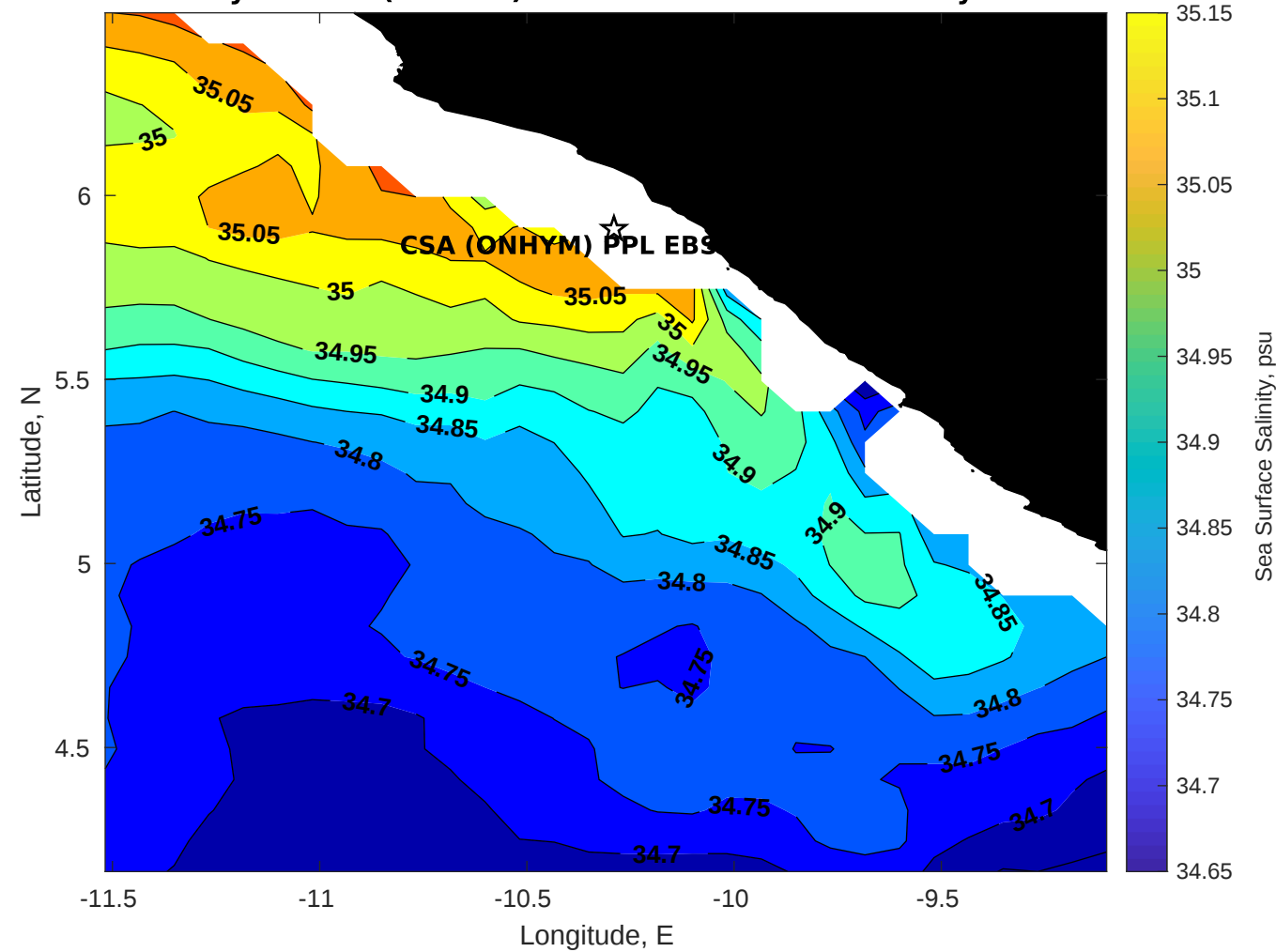
Surface Salinity for CSA (ONHYM) PPL EBS - Liberia at 24-May-2025 00:00:00
