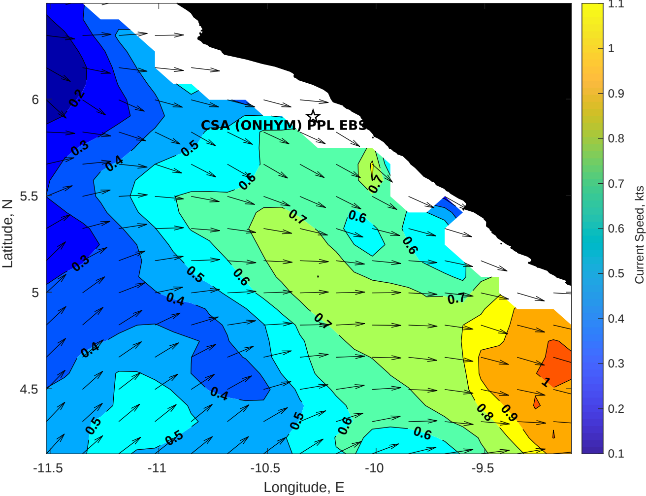
Surface Currents for CSA (ONHYM) PPL EBS - Liberia at 24-May-2025 00:00:00
