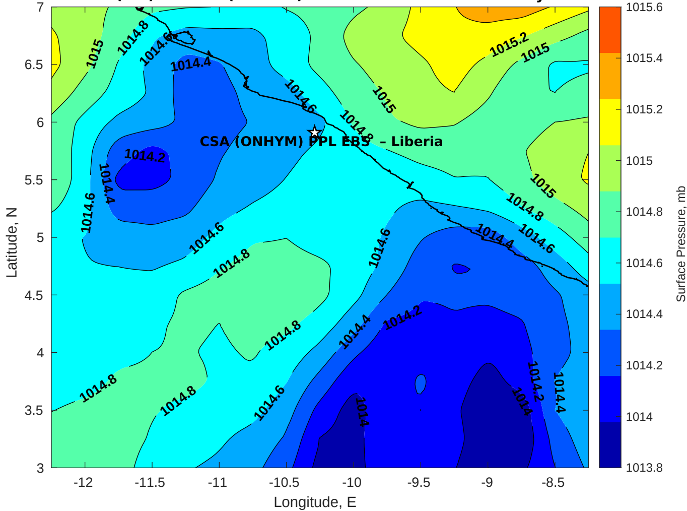
Surface Pressure (mb) for CSA (ONHYM) PPL EBS - Liberia at 25-May-2025 00:00:00
