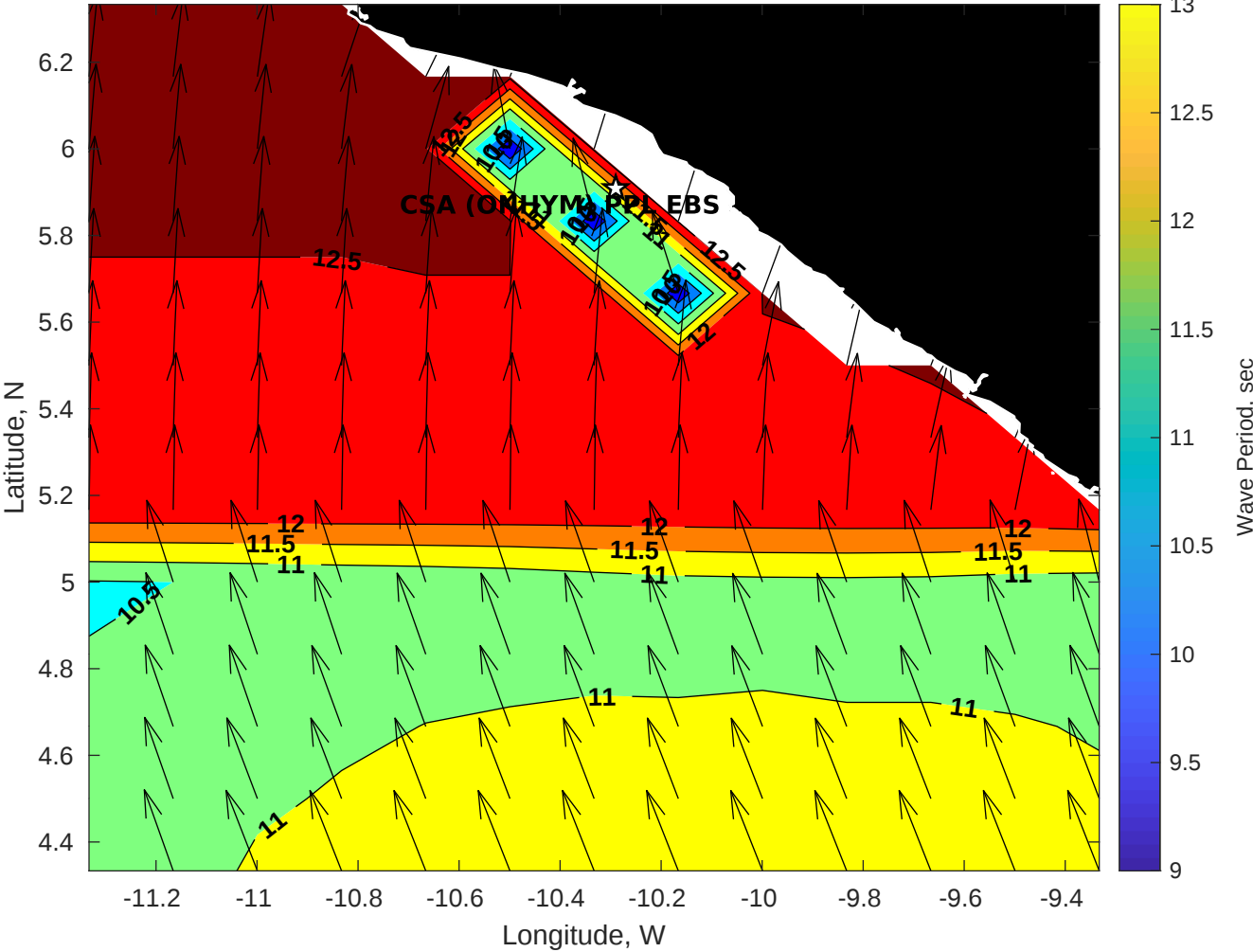
Wave Period (sec) for CSA (ONHYM) PPL EBS - Liberia at 25-May-2025 09:00:00
