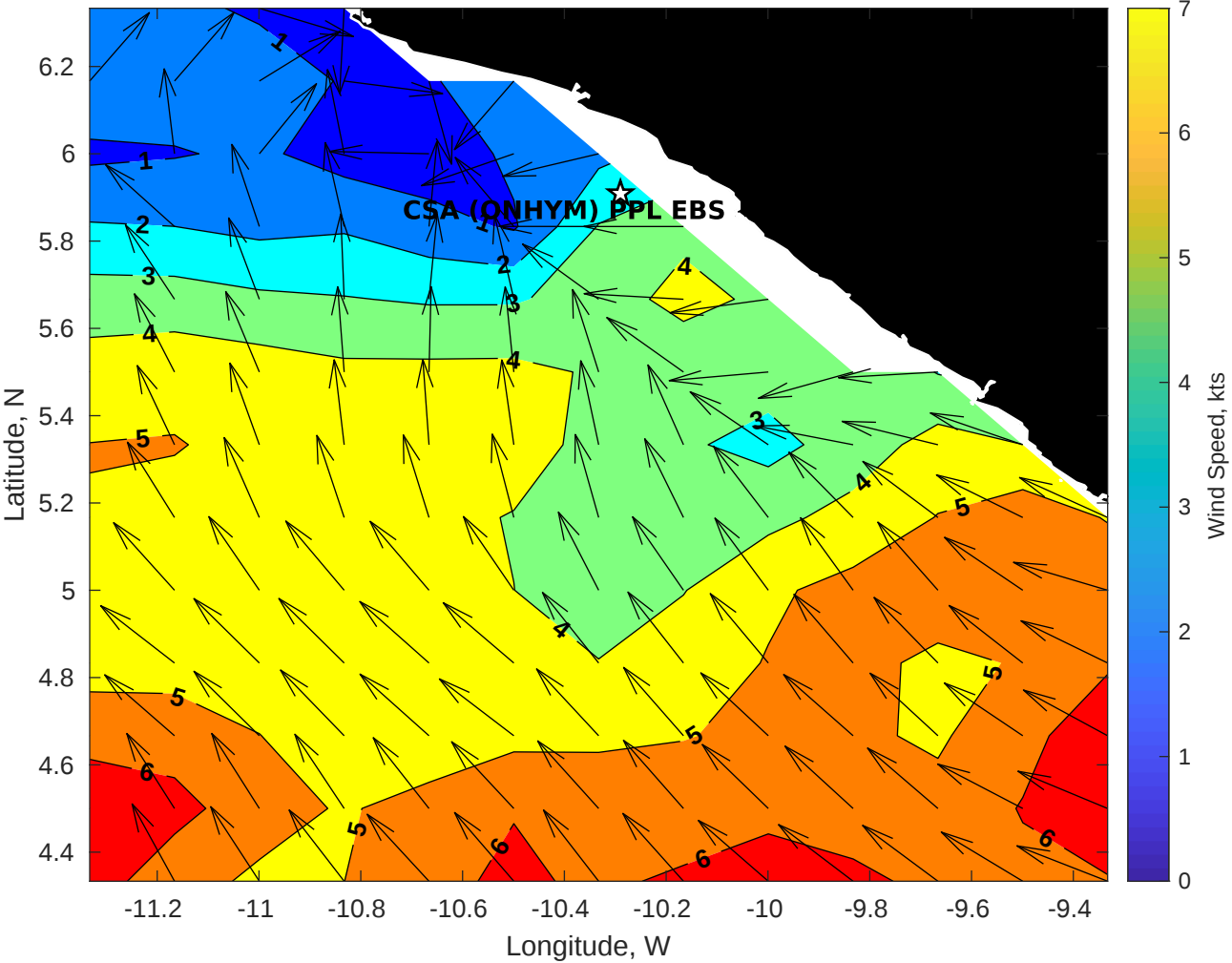
Winds (kts) for CSA (ONHYM) PPL EBS - Liberia at 25-May-2025 09:00:00
