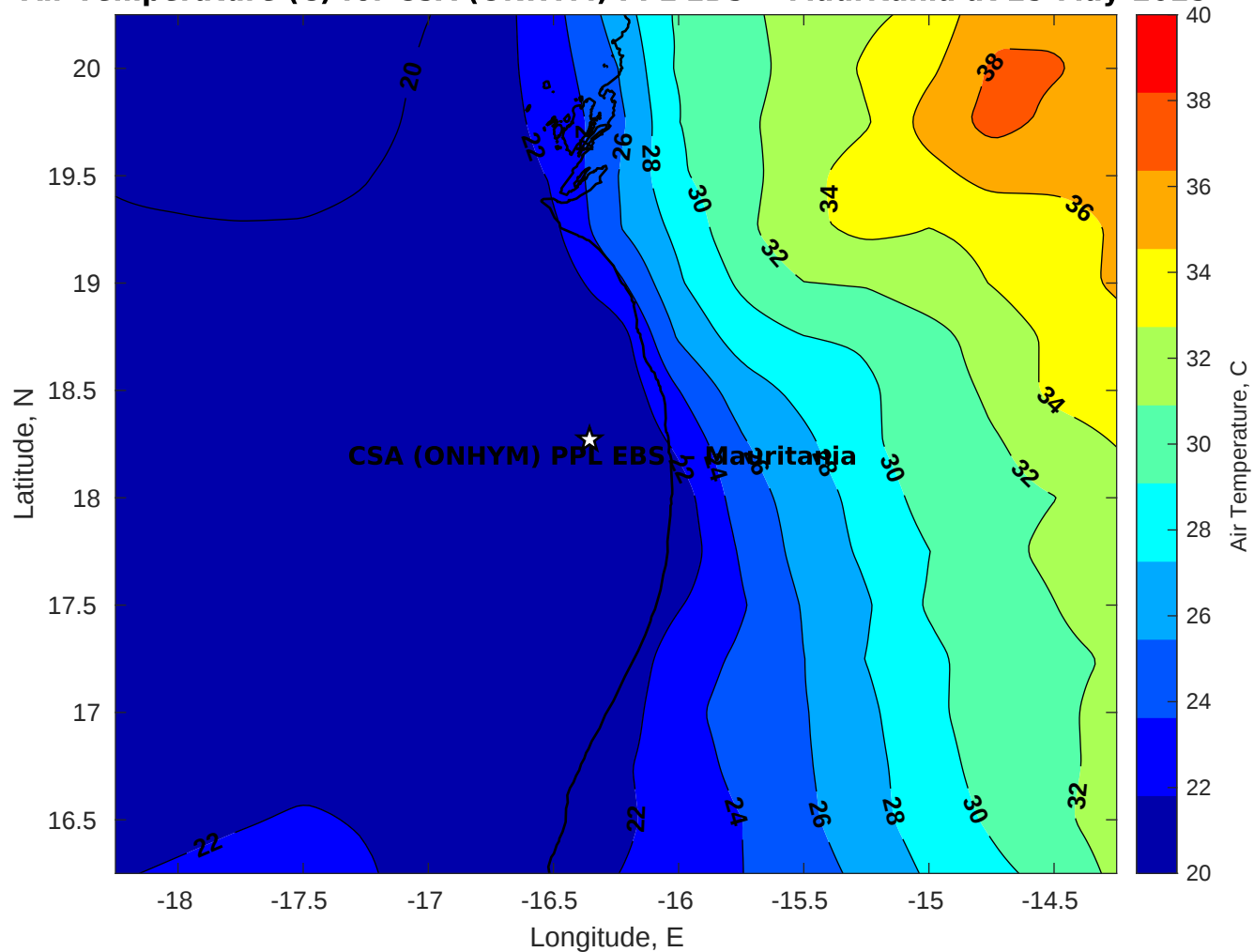
Air Temperature (C) for CSA (ONHYM) PPL EBS - Mauritania at 25-May-2025
