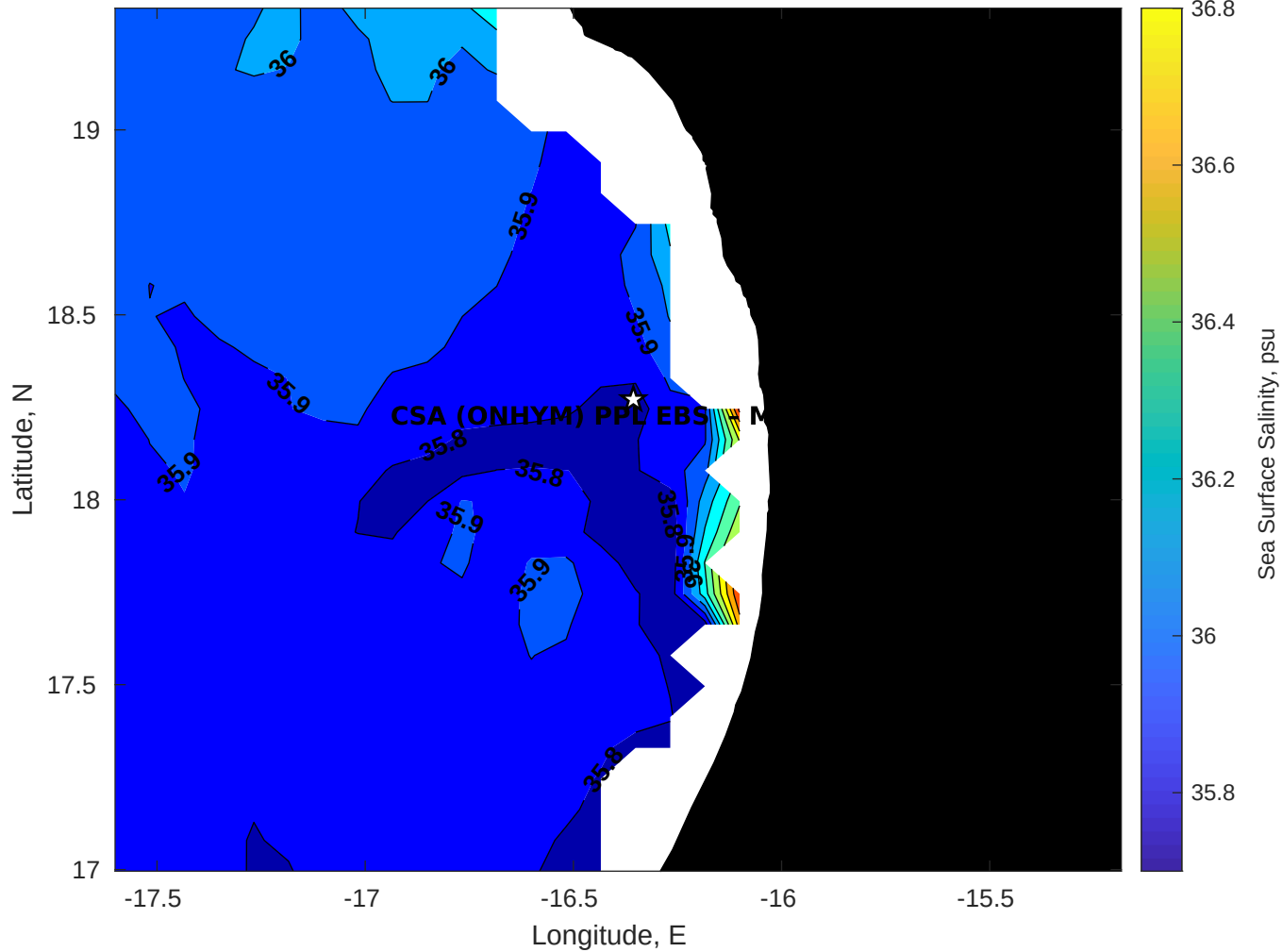
Surface Salinity for CSA (ONHYM) PPL EBS - Mauritania at 24-May-2025 00:00:00
