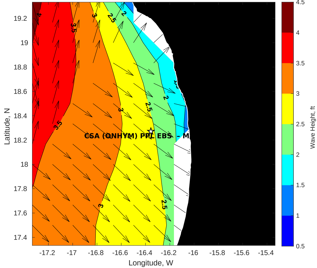
Wave Height (ft) for CSA (ONHYM) PPL EBS - Mauritania at 25-May-2025 09:00:00
