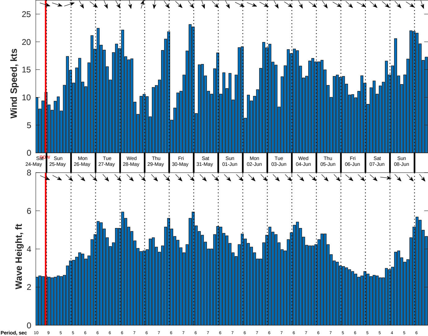
Wind & Wave Forecast for CSA (ONHYM) PPL EBS - Mauritania from 24-May-2025 13:00:00 to 09-Jun-2025 13:00:00
