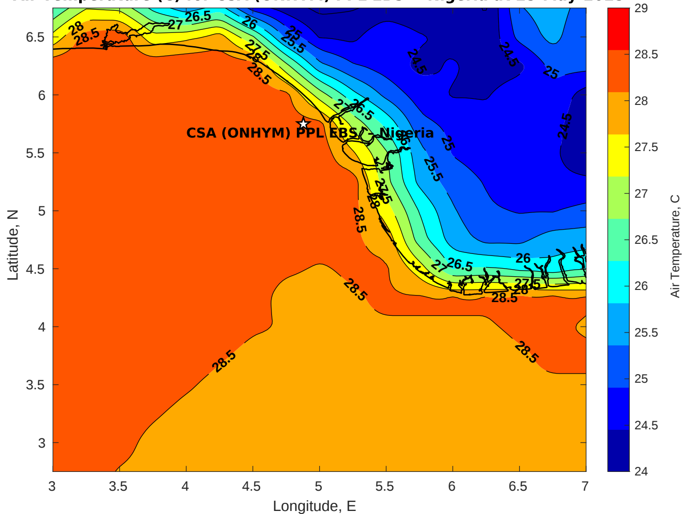
Air Temperature (C) for CSA (ONHYM) PPL EBS - Nigeria at 25-May-2025
