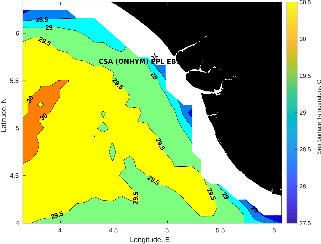
SST for CSA (ONHYM) PPL EBS - Nigeria at 24-May-2025 00:00:00
