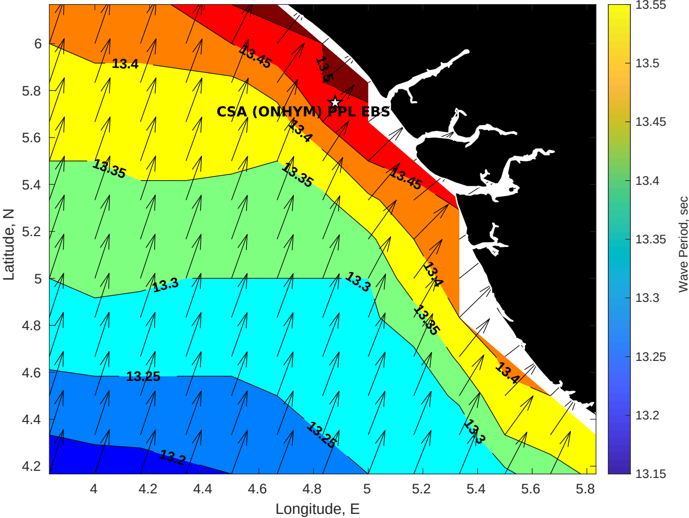
Wave Period (sec) for CSA (ONHYM) PPL EBS - Nigeria at 25-May-2025 09:00:00
