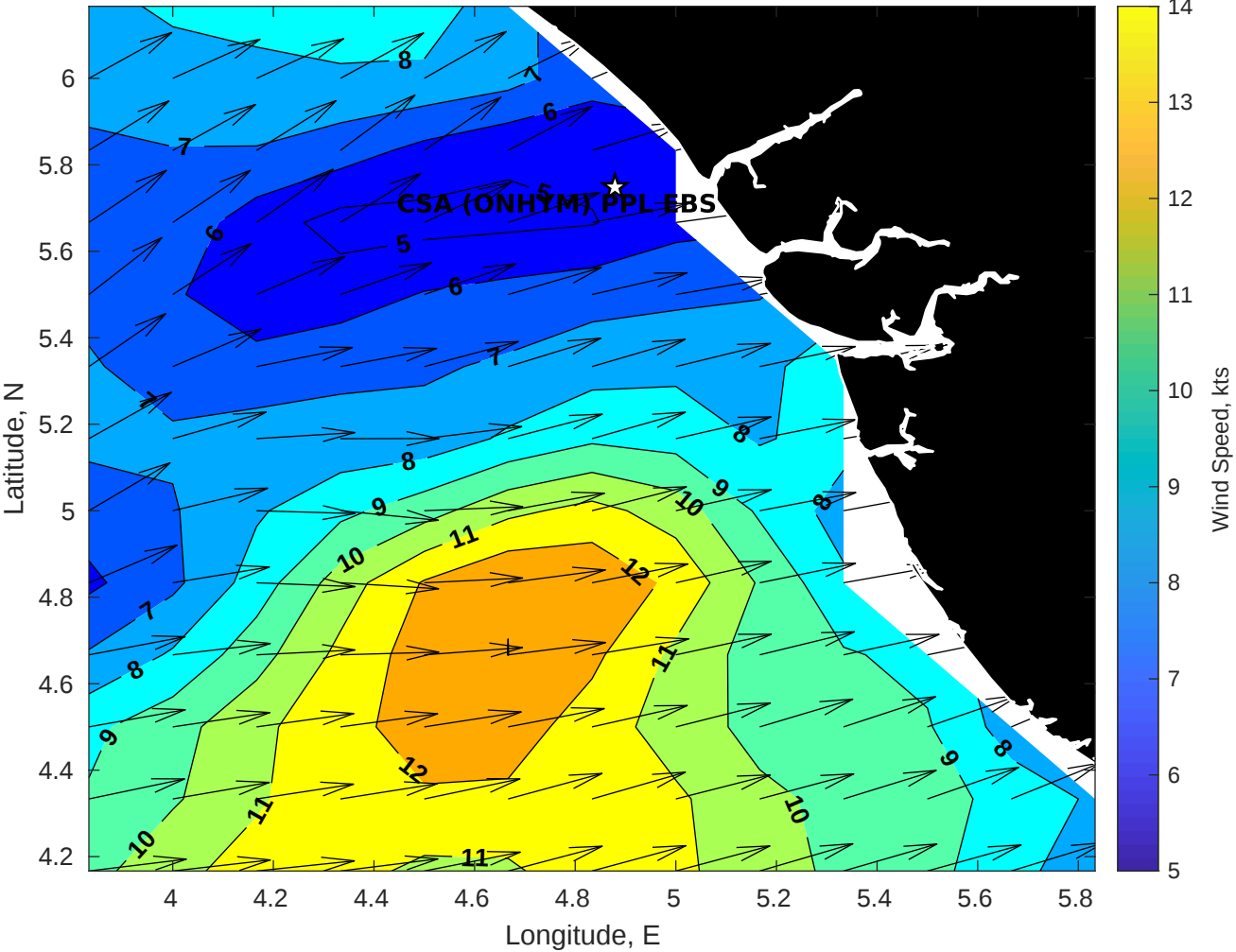
Winds (kts) for CSA (ONHYM) PPL EBS - Nigeria at 25-May-2025 09:00:00
