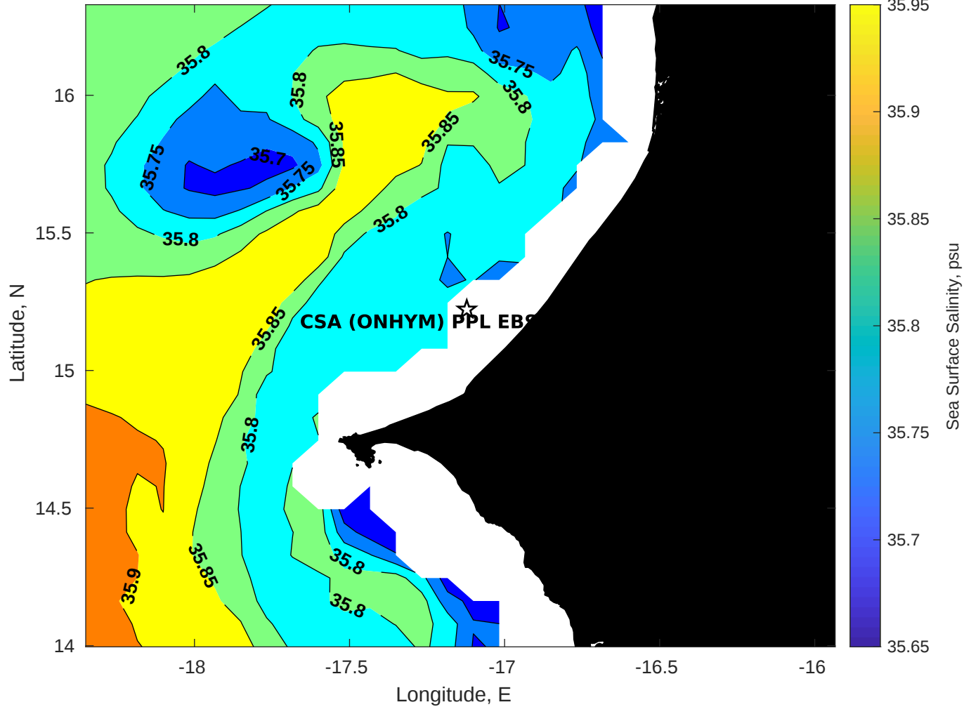
Surface Salinity for CSA (ONHYM) PPL EBS - Senegal at 24-May-2025 00:00:00
