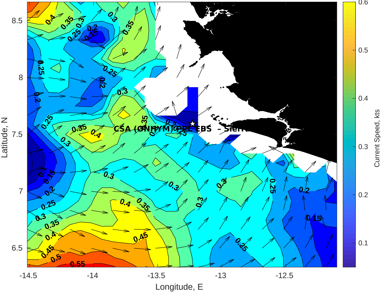
Surface Currents for CSA (ONHYM) PPL EBS - Sierra Leone at 24-May-2025 00:00:00
