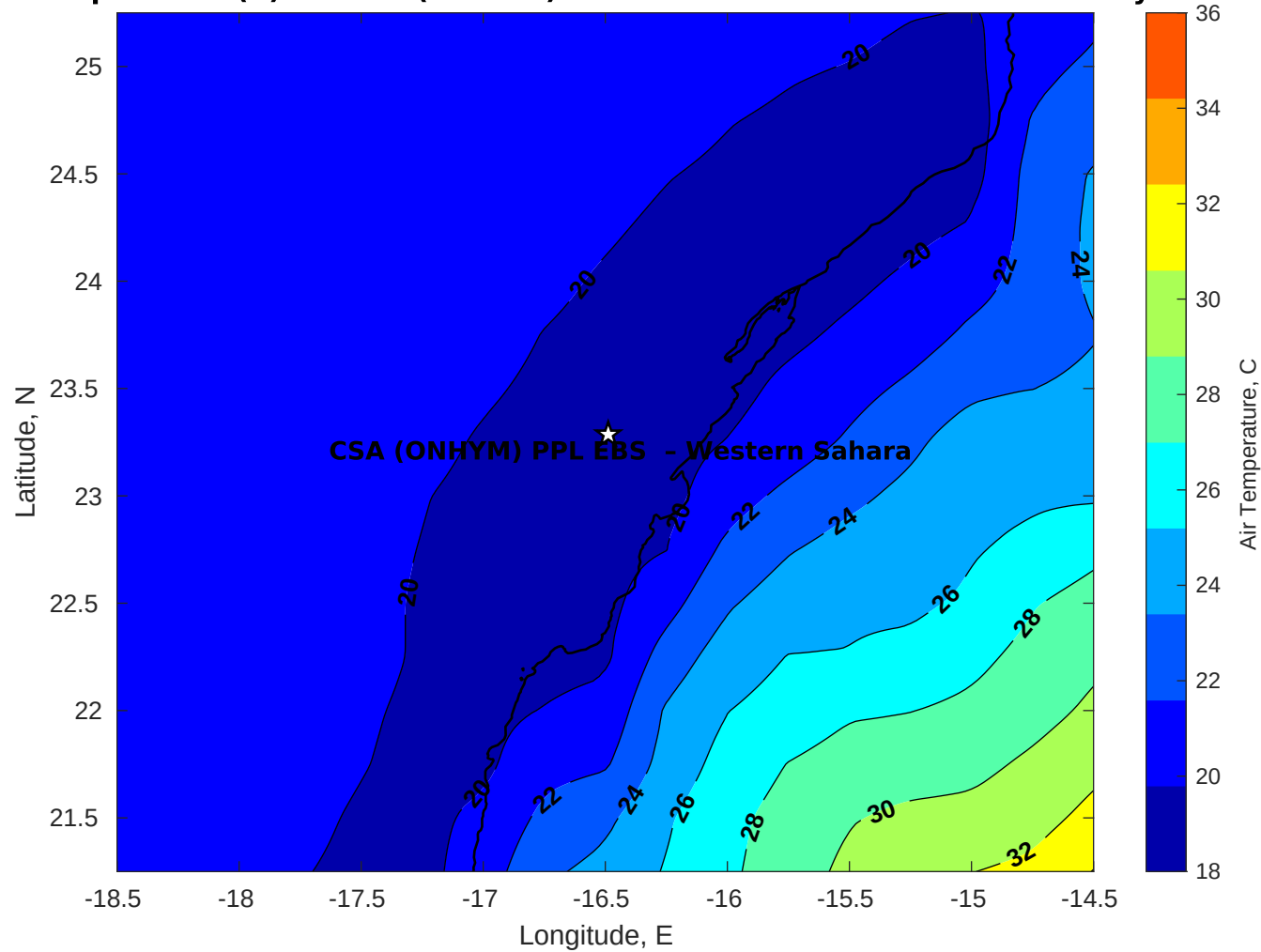
Air Temperature (C) for CSA (ONHYM) PPL EBS - Western Sahara at 25-May-2025
