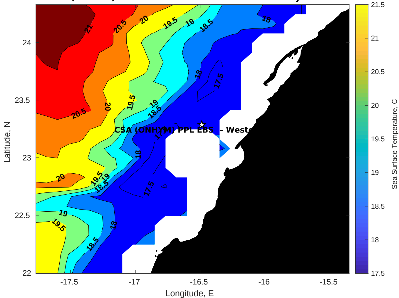
SST for CSA (ONHYM) PPL EBS - Western Sahara at 24-May-2025 00:00:00
