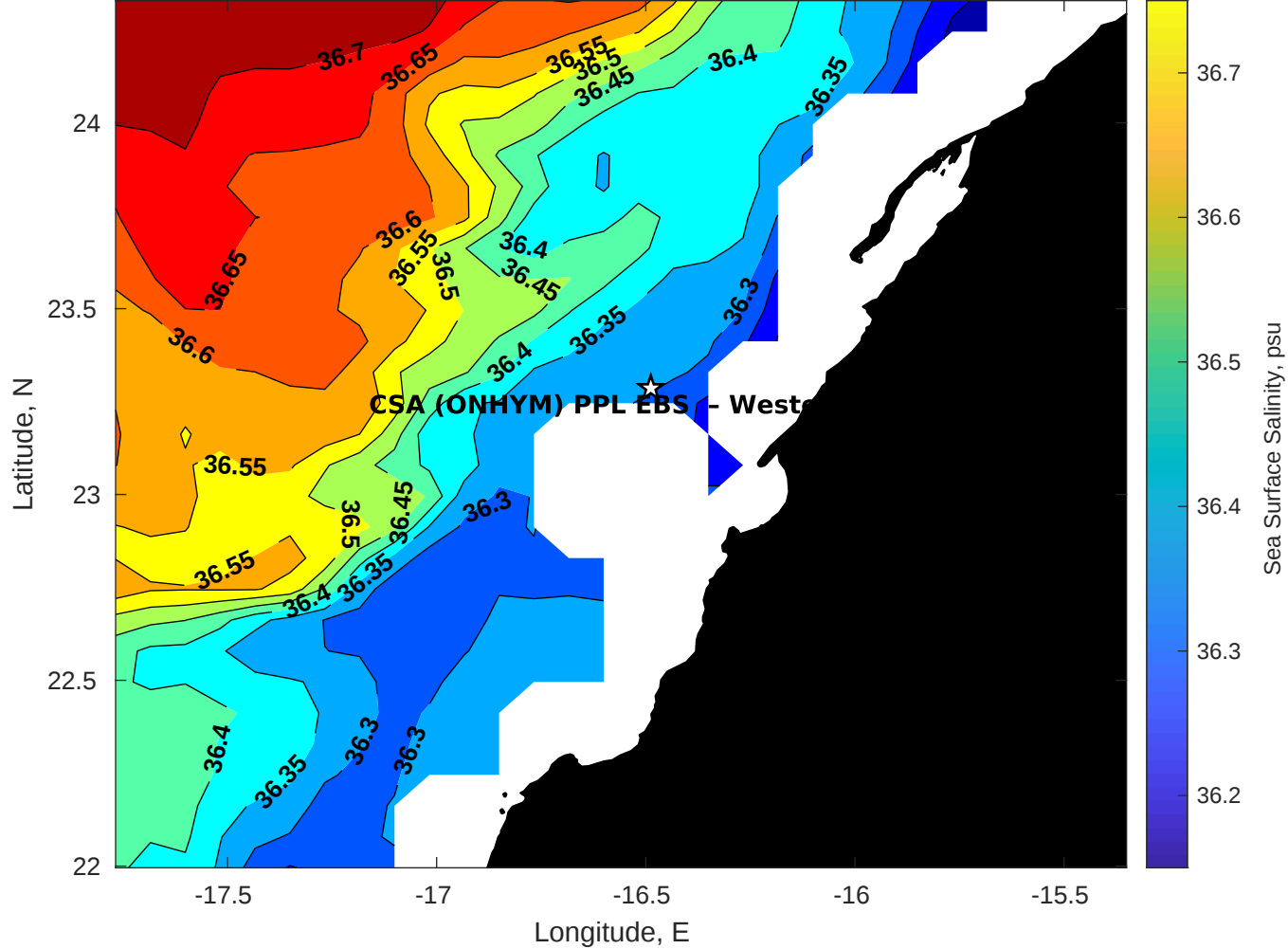
Surface Salinity for CSA (ONHYM) PPL EBS - Western Sahara at 24-May-2025 00:00:00
