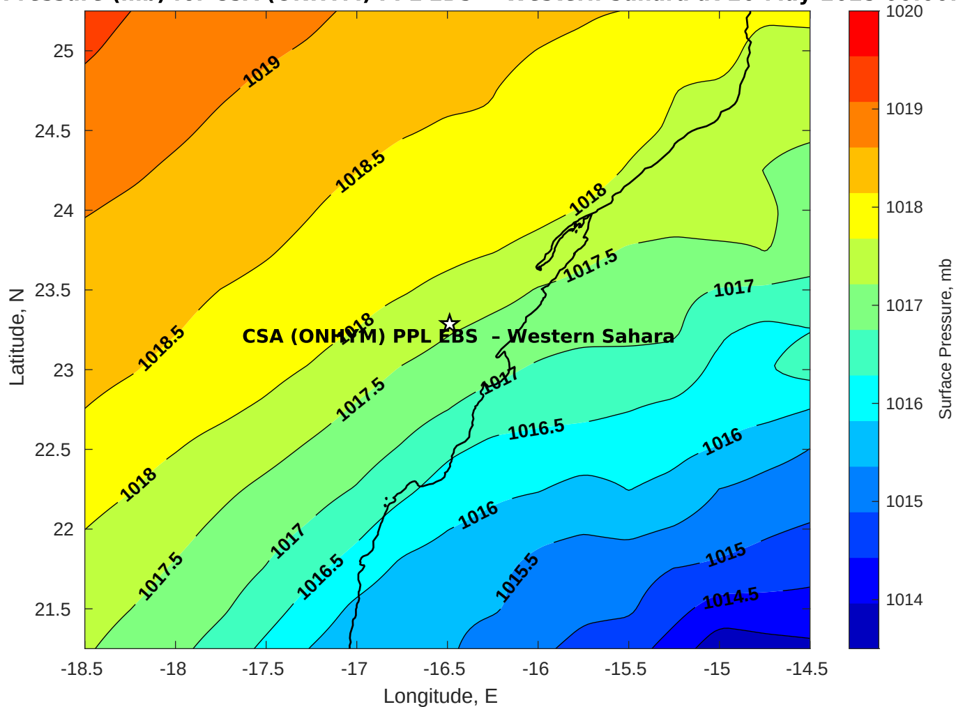
Surface Pressure (mb) for CSA (ONHYM) PPL EBS - Western Sahara at 26-May-2025 00:00:00
