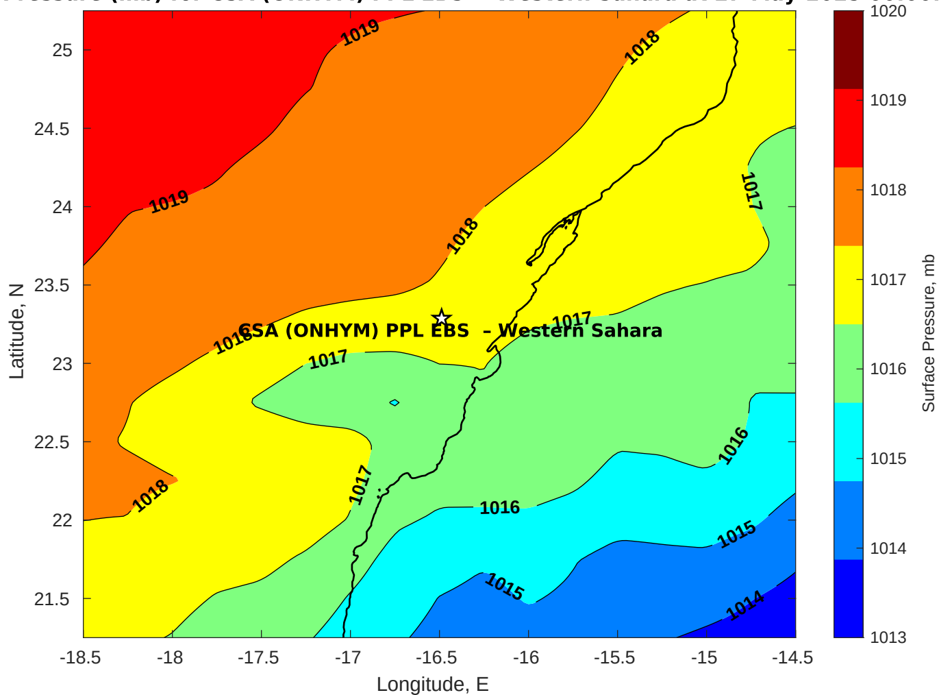
Surface Pressure (mb) for CSA (ONHYM) PPL EBS - Western Sahara at 27-May-2025 00:00:00
