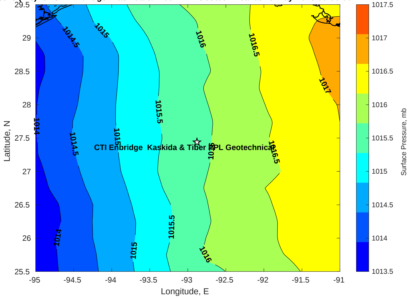
Surface Pressure (mb) for CTI Enbridge Kaskida & Tiber PPL Geotechnical at 25-May-2025 00:00:00
