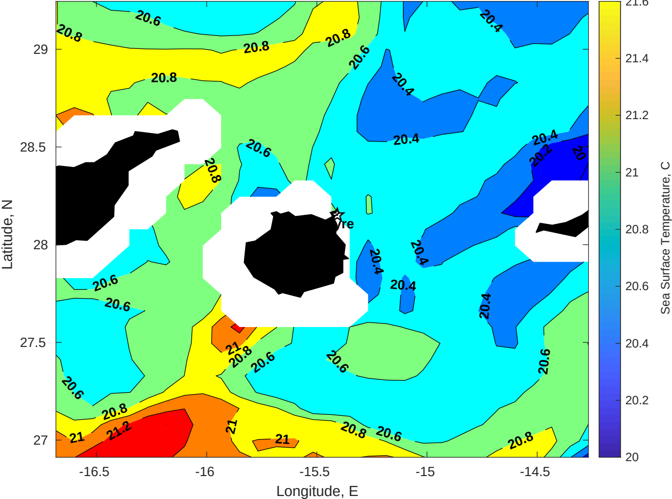
SST for Gyre at 24-May-2025 00:00:00
