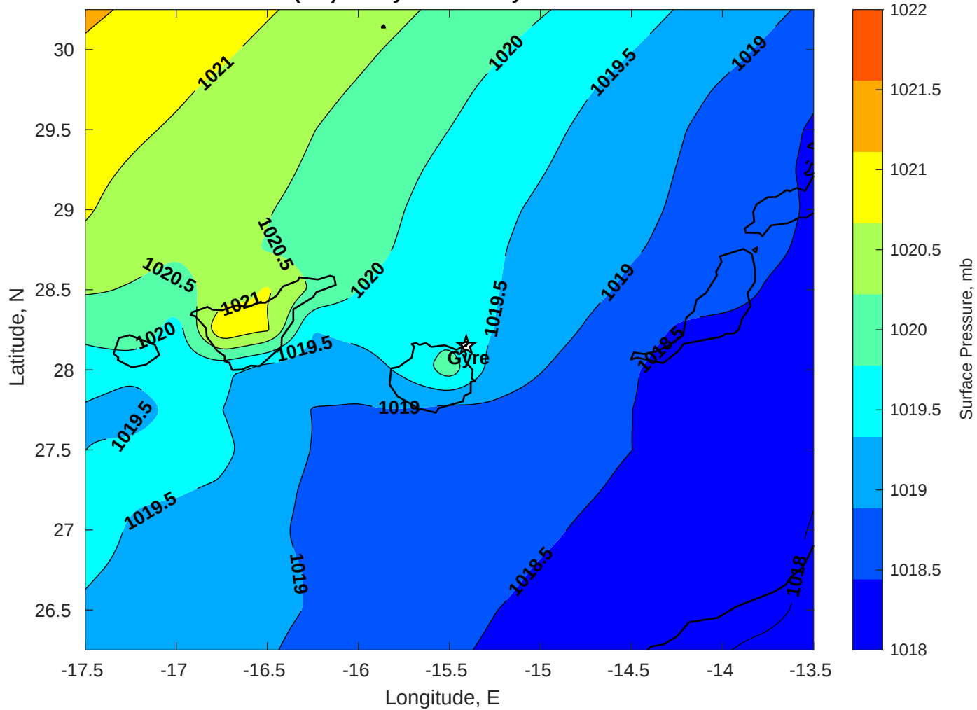
Surface Pressure (mb) for Gyre at 26-May-2025 00:00:00
