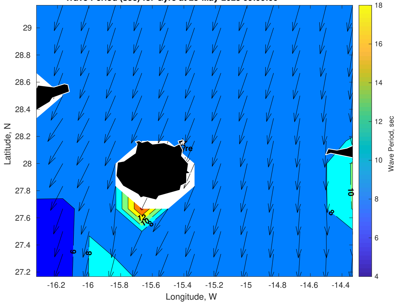
Wave Period (sec) for Gyre at 25-May-2025 09:00:00
