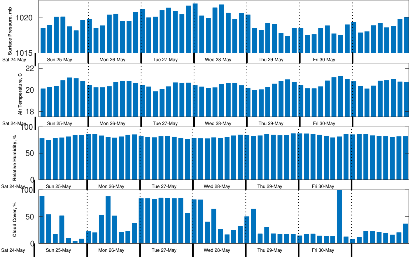
Met Forecast for Gyre from 24-May-2025 23:00:00 to 31-May-2025 23:00:00
