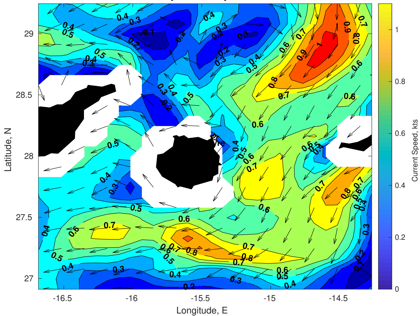
Surface Currents for Gyre at 24-May-2025 00:00:00
