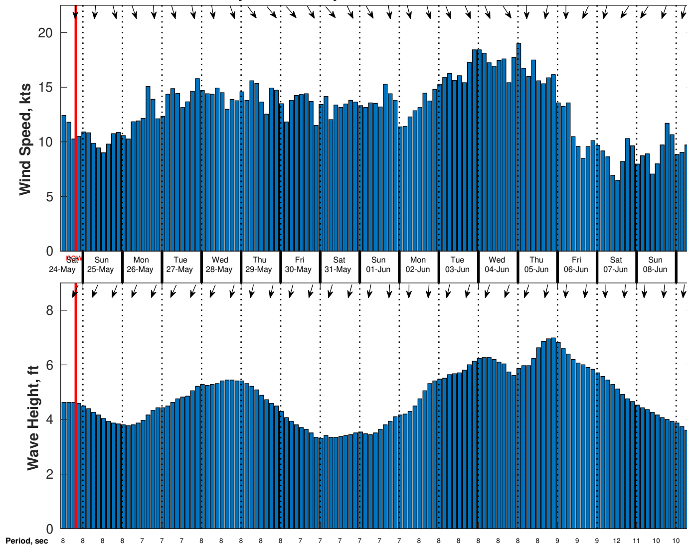
Wind & Wave Forecast for Gyre from 24-May-2025 11:00:00 to 09-Jun-2025 11:00:00
