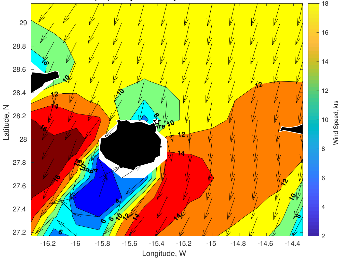
Winds (kts) for Gyre at 25-May-2025 09:00:00
