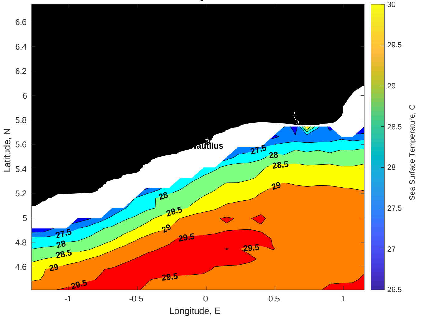
SST for Nautilus at 24-May-2025 00:00:00
