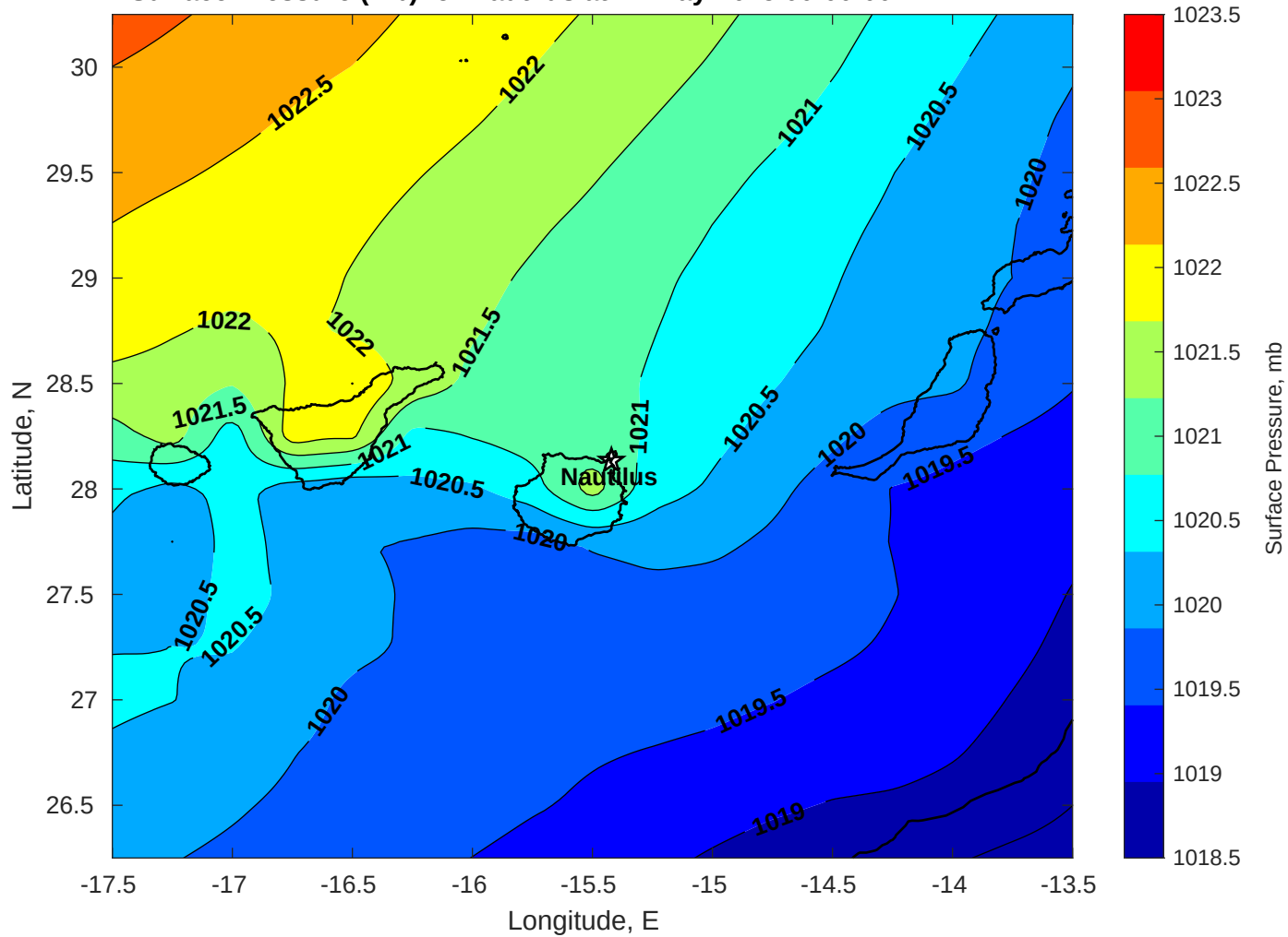
Surface Pressure (mb) for Nautilus at 27-May-2025 00:00:00
