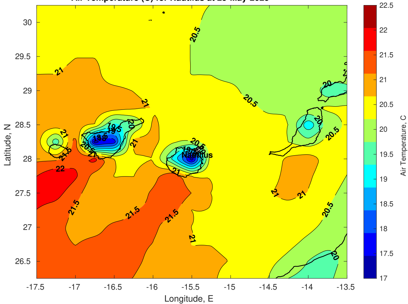
Air Temperature (C) for Nautilus at 25-May-2025
