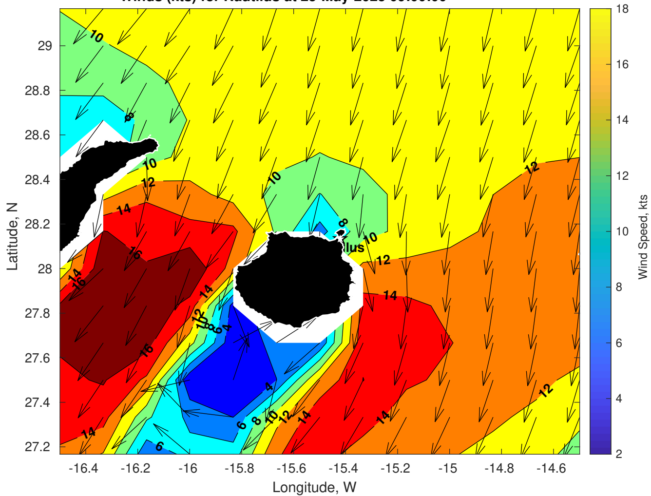
Winds (kts) for Nautilus at 25-May-2025 09:00:00
