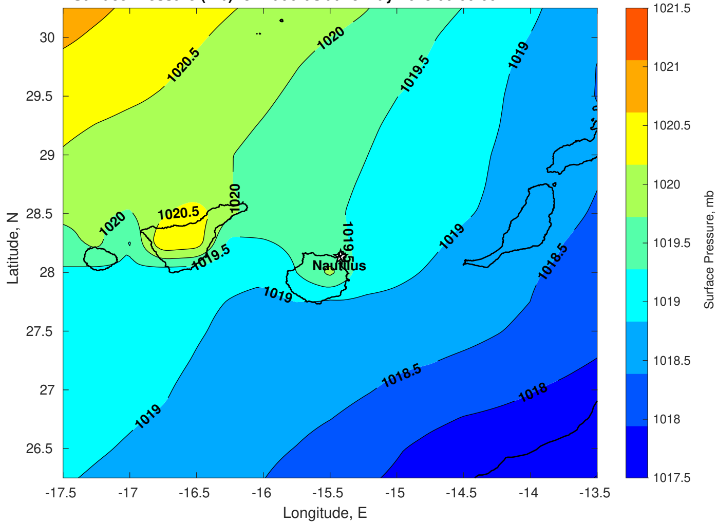
Surface Pressure (mb) for Nautilus at 25-May-2025 00:00:00
