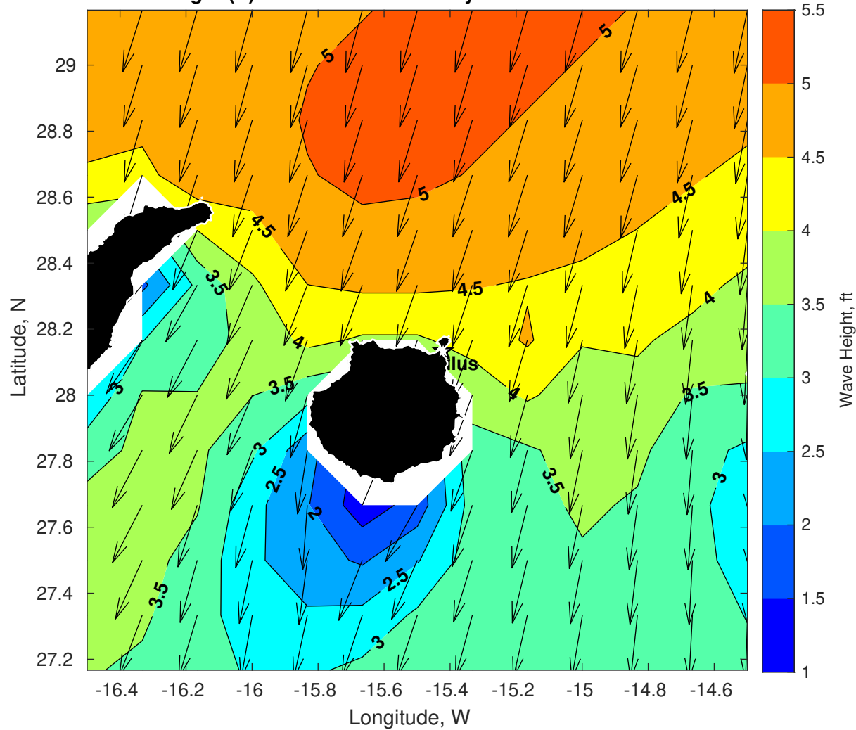
Wave Height (ft) for Nautilus at 25-May-2025 09:00:00
