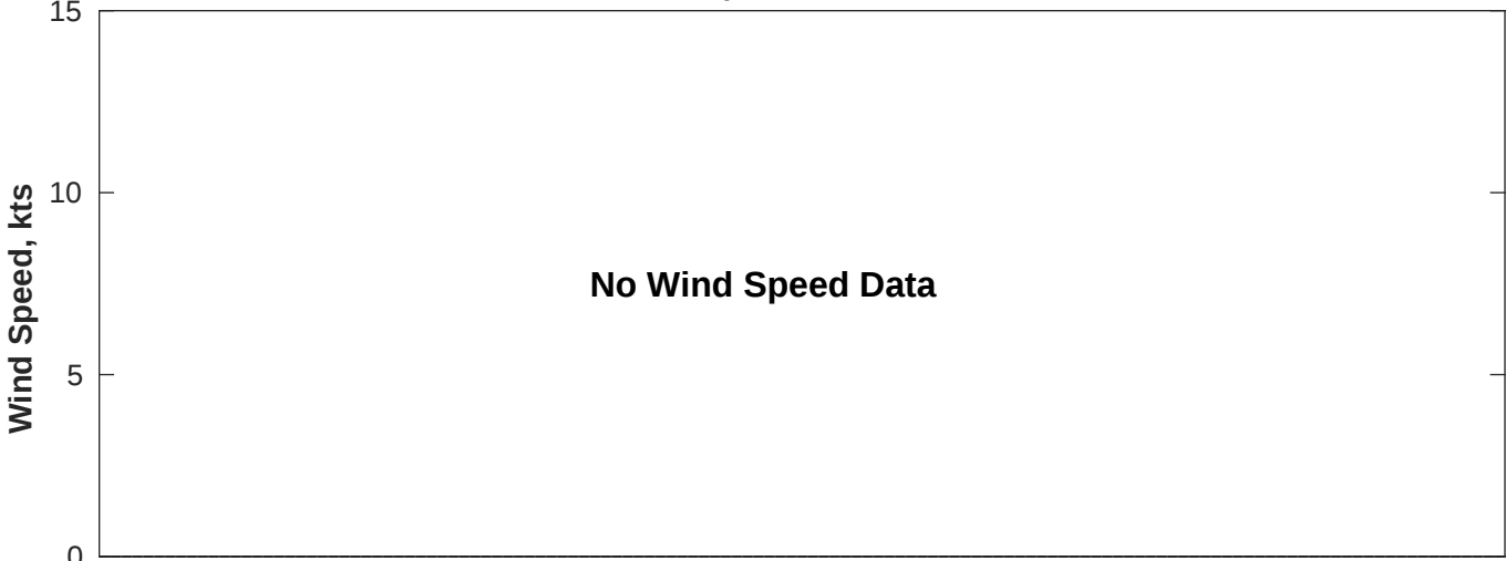
Wind & Wave Forecast for Nautilus from 24-May-2025 14:00:00 to 09-Jun-2025 14:00:00
