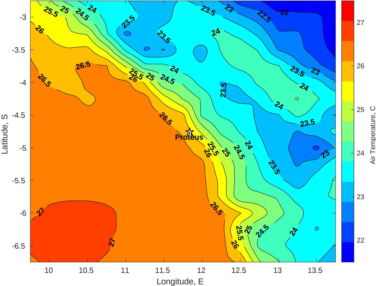
Air Temperature (C) for Proteus at 25-May-2025
