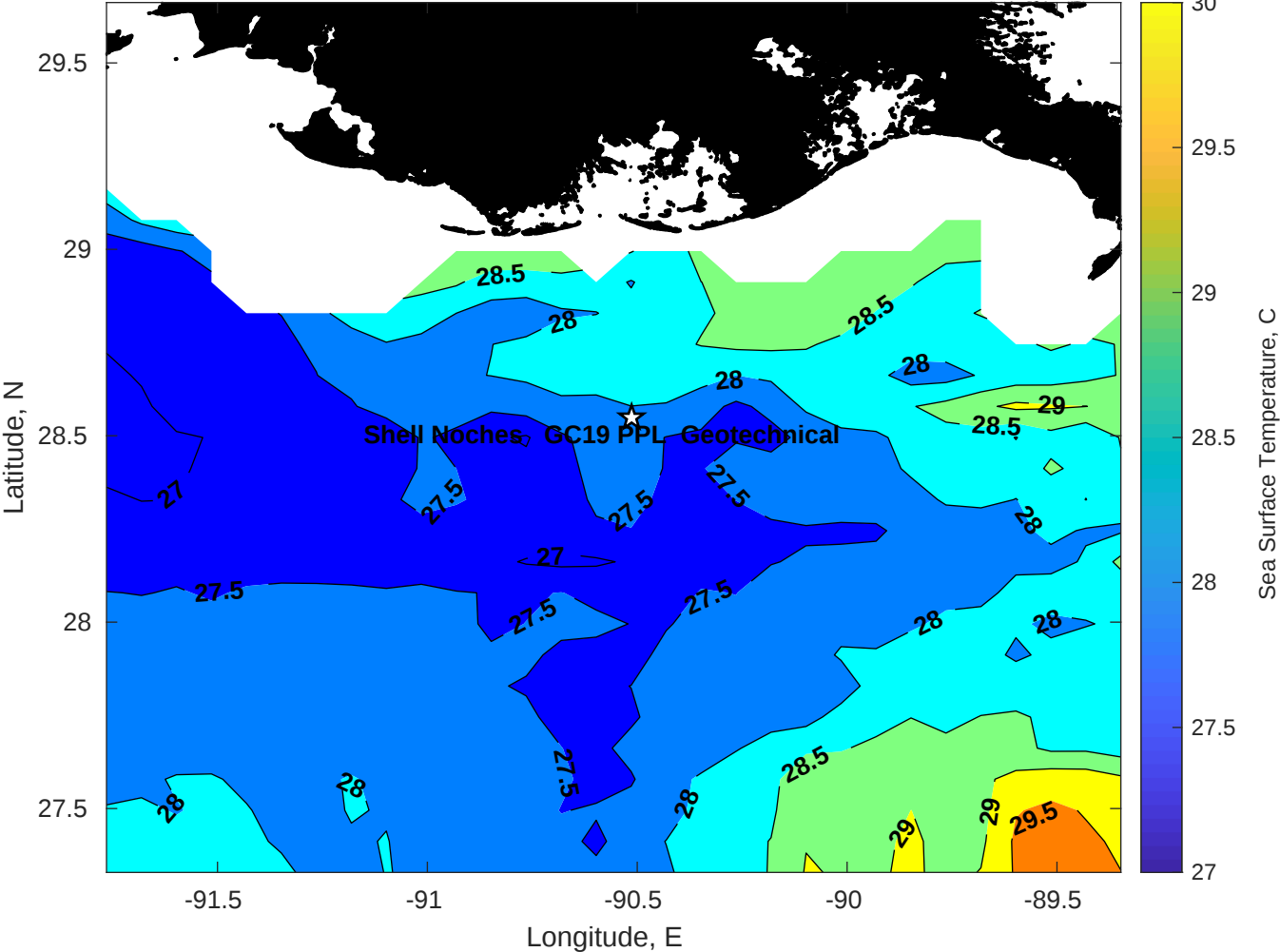
SST for Shell Noches GC19 PPL Geotechnical at 24-May-2025 00:00:00
