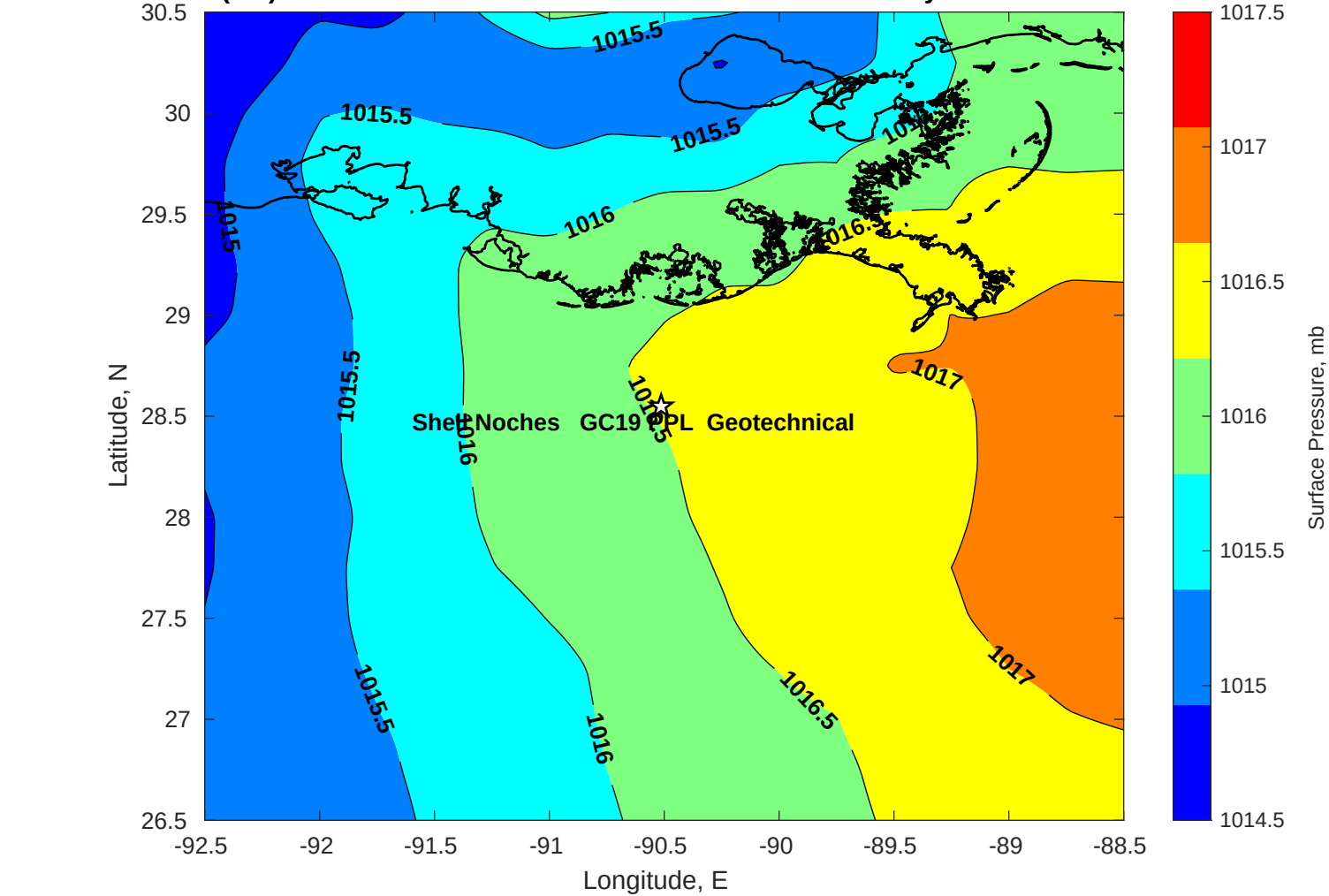
Surface Pressure (mb) for Shell Noches GC19 PPL Geotechnical at 26-May-2025 00:00:00
